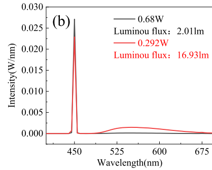
Fig. 5. The SPDs of 10% YAG: Ce^{3+} phosphor/silicone composite measured under (a) R-mode; and (b) T-mode integrating sphere 2.
