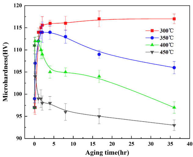
Figure 7 Microhardness-time curves for the Ca-modified Al–Mg–Sc alloy aged at 300 °C ~ 450 °C.
