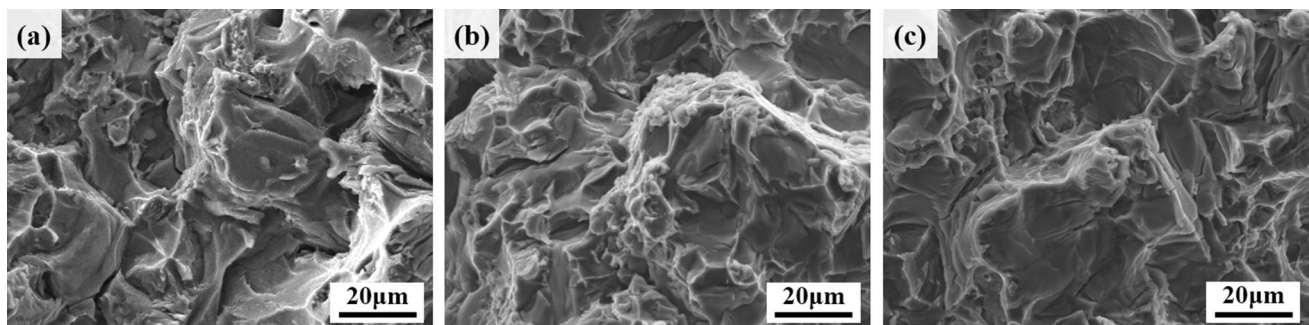
Figure 9 Fracture surfaces of Ca-modified Al–Mg–Sc specimens aged at 300 °C for 4h, a tested at room temperature, b at 150 °C, c at 300 °C.
