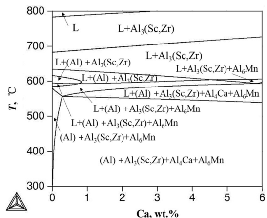
Figure 1 Vertical section of Al–Mg–Sc–Zr–Mn–Ca system at 5%Mg, 0.5%Sc, 0.2%Zr and 0.5%Mn (wt.%).
