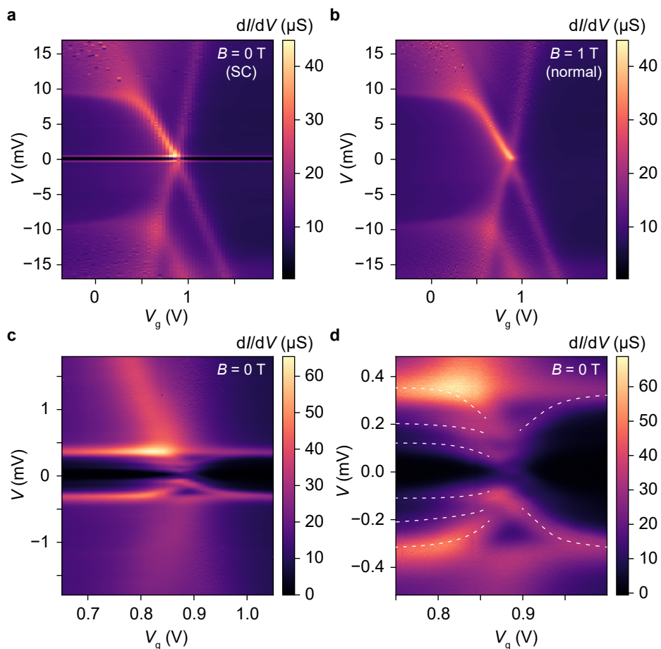
Figure 6.11: Transport measurements of a NbTiN-based proximity-induced superconducting junction exhibiting Coulomb blockade. a. Stability diagram of the superconducting state ( B = 0 T) showing a single charge resonance and a superconducting gap at low bias. Cotunneling excitation lines appear at V = \pm 9 mV. b. Stability diagram of the normal state ( B = 1 T) where no superconducting gap is present. c. Detailed stability diagram of the region around the charge resonance showing a superconducting gap at V \approx \pm 0.3 mV along with the appearance of gate-dependent subgap resonances. d. Closeup of c in which the subgap resonances are highlighted by white dashed lines.
