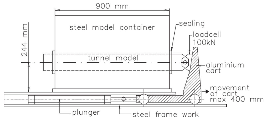
Fig. 2. Sketch of centrifuge tests in Bezuïjen and Brassinga (2006).
