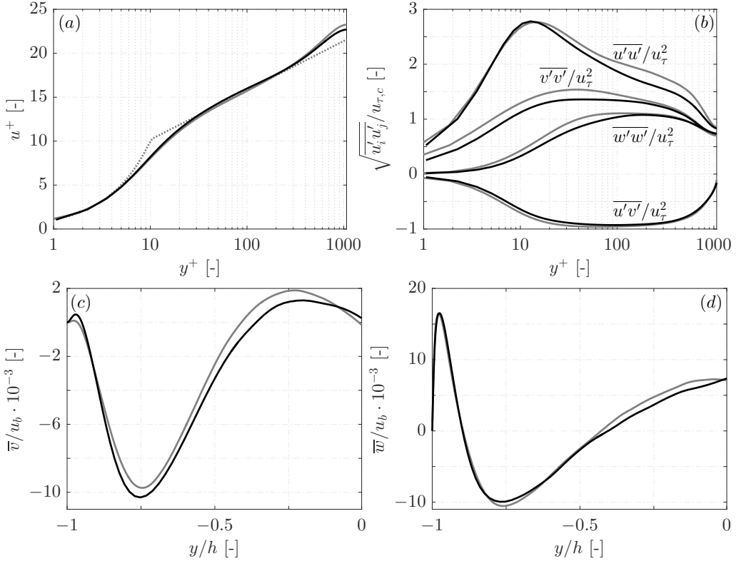
Figure 27: Profiles of (a) mean streamwise velocity and (b) Reynolds stresses along the duct midplane at z = 0 , and (c)/(d) secondary flow velocities at z = 0.75 for the LES (—) and DNS (—) results of the adiabatic square duct. In (a) the analytical law of the wall ( u^+ = 1/0.41 \cdot \ln y^+ + 4.55 ) is represented by (.....).
