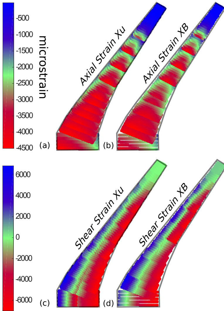
Fig. 11 Top skin axial (a,b) and shear (c,d) strains for the unblended and blended designs
