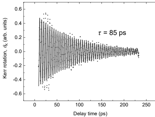
Figure 7.5: Extracting the spin-wave propagation distance. Time-resolved polarization rotation originating from a propagating magnon, as obtained in the reflection geometry. The solid line represents a best fit of a damped sine, giving a lifetime \tau of about 85 ps. With the largest estimated group velocities v_g of the measured magnons of about 13 km/s, this gives a propagation distance l_c = v_g \tau = 1.1 \mu\text{m} .
