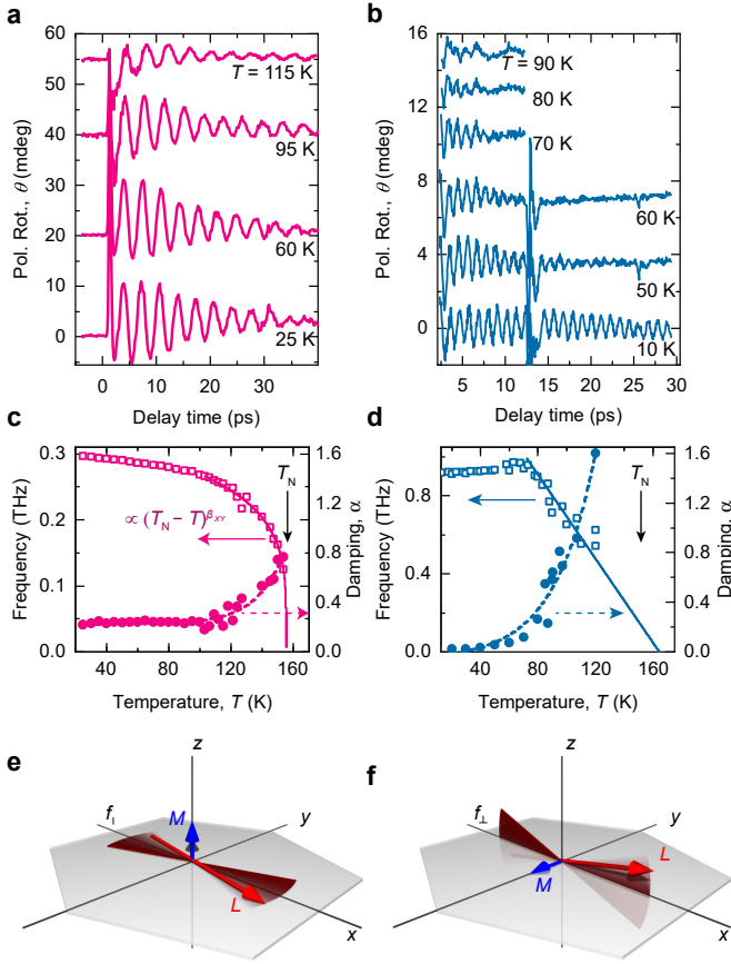
Figure 6.4: Critical behavior of the light-induced coherent dynamics. a, b , Temperature dependence of the time-resolved polarization rotation after pump-induced excitation with photon energies of 1.08 eV ( a ) and 0.2 eV ( b ). Irregularities around a time delay of 13 ps in ( b ) are related to an artifact of the measurement setup. c, d , Frequency (left axis) and damping factor \alpha (right axis) of the oscillations as extracted from the damped sine fits of the time-domain data in panel a and b . The solid lines represent the best fit of (T_N - T)^\beta ( c ), which gives T_N = (15 \pm 5) K and \beta = 0.23 , and a linear function ( d ) to the frequency data. e, f , Schematics of the in-plane ( e ) and out-of-plane ( f ) magnon modes.
