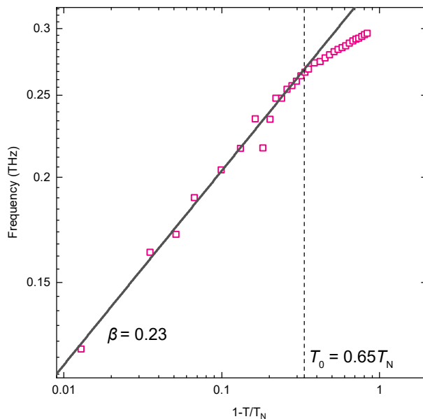
Figure 6.8: Temperature-dependence. The magnon frequency f_1 for different temperatures on a \log\text{-}\log scale. The solid line is a linear fit to the high-temperature datapoints close to the Néel temperature T_N and provides the value of the critical exponent \beta = 0.23 .
