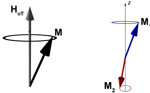
Figure 2.4: Uniform spin precession. a , In ferromagnets, the net magnetization \mathbf{M} precesses around an effective magnetic field \mathbf{H}_{\text{eff}} . b , In antiferromagnets, both magnetic sublattices precess around their equilibrium direction.
