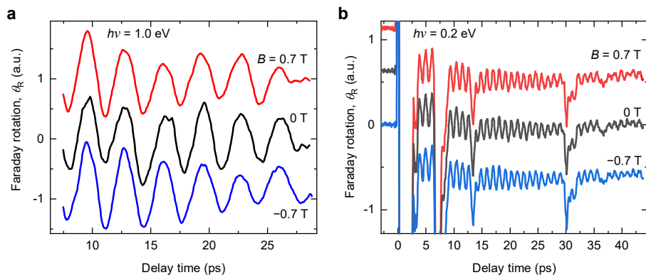
Figure 6.7: Magnetic field dependence. a, b , Pump-induced polarization rotation for different values of the external magnetic field applied in the sample ( ab ) plane, after excitation at a pump photon energy of 1.0 eV ( a ) and 0.2 eV ( b ). The traces for different magnetic fields are shifted for clarity.
