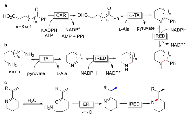
Figure 29. a) Example of an enzymatic cascade with IREDs to obtain chiral piperidines. CAR = carboxylic acid reductase. b,c) Bi-enzymatic cascade with b) a putrescine transaminase and IRED to obtain piperidines, c) ER and IRED for the selective reduction of enamines to chiral piperidines derivatives.
