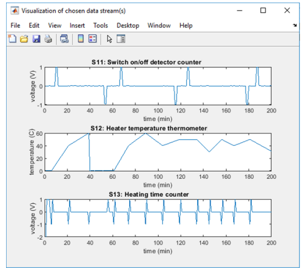
Fig. 5. Visualization of combined sensors 11, 12 and 13
