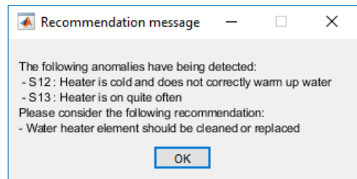
Fig. 6. Recommendation message communicated to the designer
