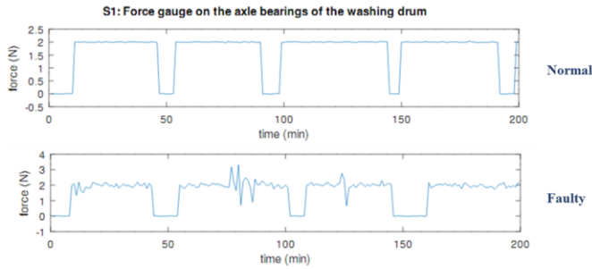
Fig. 3. Visual representation of the normal and faulty behavior of sensor 1
