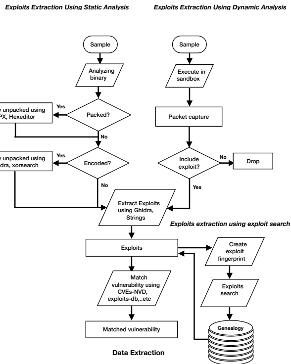
Figure 1: Analysis pipeline. We extract exploits using static and dynamic analysis from samples collected from 2018 to 2020 to create signatures, which we then match against a Genealogy dataset of unpacked samples from 2015 to 2018.
