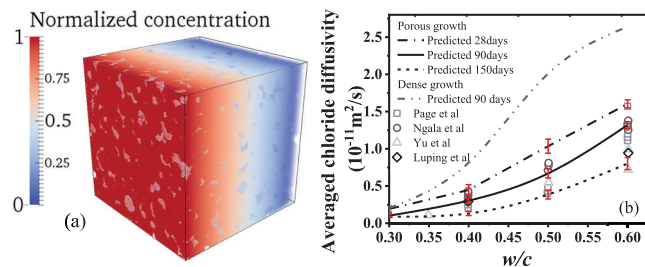
FIGURE 17 Results of (a) normalized concentration distribution at the steady-state diffusion, (b) predicted chloride diffusion coefficient with different w/c ratios (average results of 10 repetitions with error bars).
