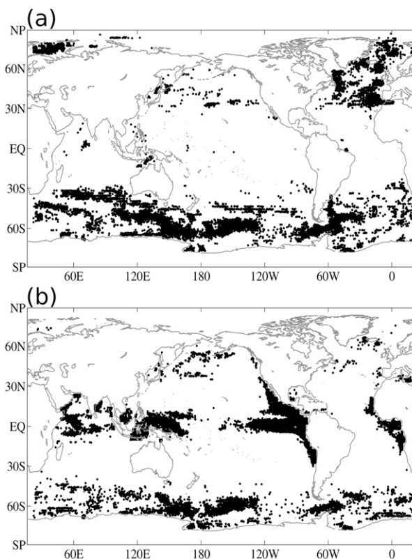
FIG. 3. Surface hitting locations for deep North Pacific particles (a) showing where particles last hit the surface before being transported to the DNP (i.e., surface locations where tracers enter the deep Pacific ocean) and (b) showing where particles in the DNP will first hit the surface (i.e., locations where deep Pacific tracers are first exposed to the atmosphere). Of initial populations of 146 340 particles, only particles with last- or first-passage times less than 3000 yr are shown.
