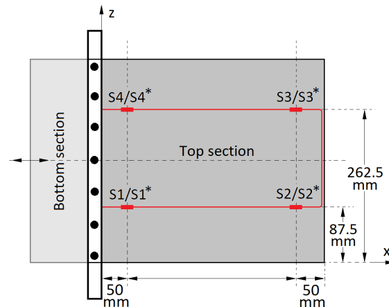
Figure 7. Top-view of the wing with the optical fibre running along the x-axis in the bulk of the top (and bottom) section(s). The grating sensors S1 , S2 , S3 and S4 are on the top section. The sensors on the bottom section are a superimposition of the top sensor positions marked with asterisks (*); (e.g., S1 directly above S1^* and so on).
