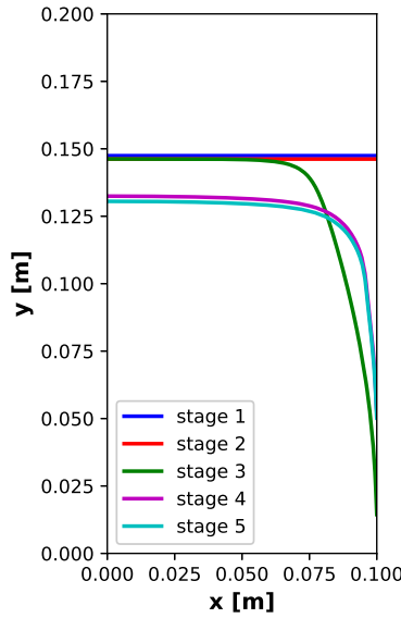
Figure 7.18: Melting front positions obtained in all stages of the benchmark by STAR-CCM+.
