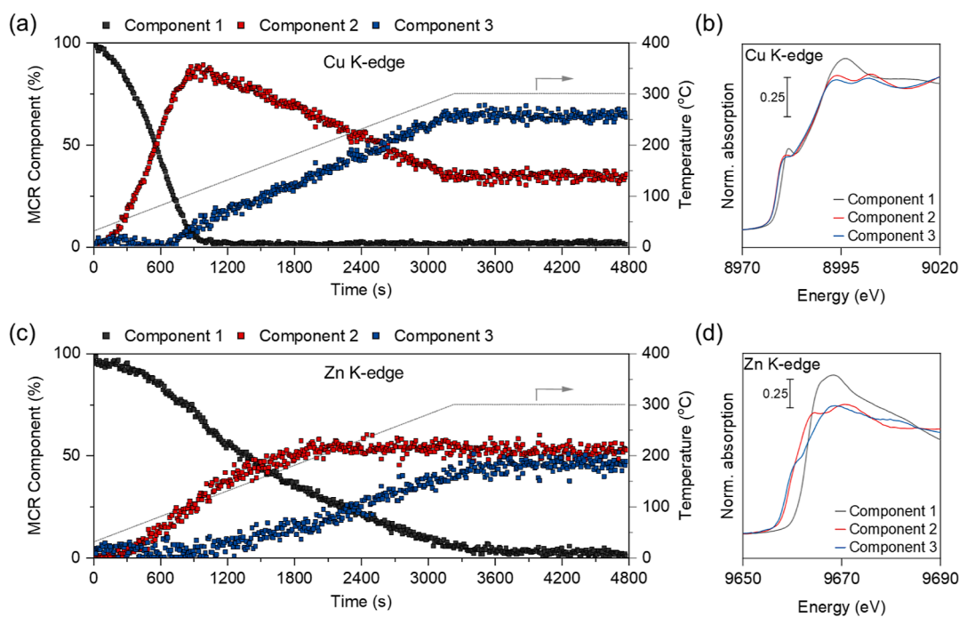
Figure 4. MCR-ALS analysis of XANES data recorded during H 2 pretreatment of passivated Cu–Zn(S)/SiO 2 with (a) extracted component fractions at the Cu K-edge as a function of time; gray trace shows temperature as a function of time; and (b) the corresponding spectrally pure components (see Figure S53 for in situ spectra). (c) Component fractions at the Zn K-edge as a function of time; gray trace shows temperature as a function of time; and (d) corresponding spectrally pure components (see Figure S57 for in situ spectra). Conditions: 3 mm quartz capillary (i.d. 2.8 mm), using ca. 20 mg of passivated Cu–Zn(S)/SiO 2 , temperature raised from room temperature to 300 °C, P = 1 bar, total flow rate 10 mL min −1 of indiluted H 2 .
