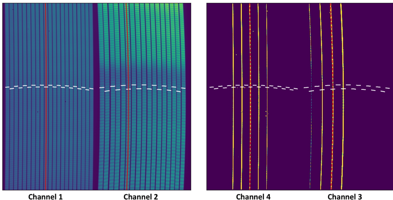
Fig. 1. Left: MRS SW detector (channels 1 and 2) illumination caused by an extended source filling the MRS FOV. Right: MRS SW detector illumination caused by a compact source. The illumination pattern along the slices follow the iso- \alpha lines (see text for details). The iso- \alpha and iso- \lambda lines are highlighted with red (iso- \alpha ) and white (iso- \lambda ) lines overlaid on the detector image.
