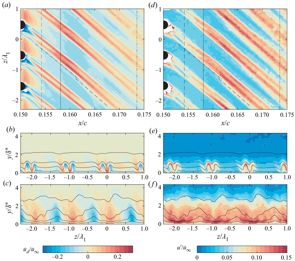
Figure 15. (a–c) Values of \bar{u}_d and (d–f) u' for forcing case \lambda_{f1} , Re_k = 330 in (a,d) the xz plane at y/\delta^* = 0.55 ; (b,e) in the yz plane at x_1 = 0.154c (vertical dashed line in a), and (c,f) at x_2 = 0.174c (vertical dash-dot line). Vertical full line in (a) at x/c = 0.158 .
