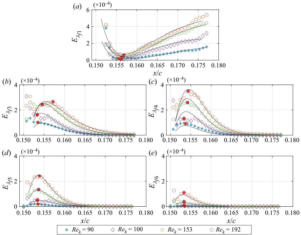
Figure 8. The E_{\lambda_{fi}}(\bar{u}) trends (symbols, 1 out of 5 shown) and maximum values (red circle) and transient growth modelling functions (black lines, White et al. 2005) at various Re_k for individual FFT modes; (a) \lambda_{f1} , (b) \lambda_{f3} , (c) \lambda_{f4} , (d) \lambda_{f5} , (e) \lambda_{f6} .
