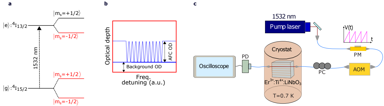
Fig. 1. a. Simplified energy level structure of the {}^4I_{15/2} \leftrightarrow {}^4I_{13/2} transition of \text{Er}^{3+} . Excited and ground levels are indicated with |e\rangle and |g\rangle , respectively, and electronic Zeeman sub-levels with |m_s = \pm 1/2\rangle . To create an atomic frequency comb (a periodic modulation of the frequency-dependent optical depth into equally-spaced narrow peaks), persistent spectral holes are created (burned) by pumping all undesired population into shelving levels, e.g. |g, m_s = +1/2\rangle . b. An example of an AFC, showing the resulting spectral population grating. c. Experimental setup. Continuous-wave light at 1532 nm wavelength is directed through a phase-modulator (PM) and an acousto-optic modulator (AOM), which allow frequency and intensity modulation. After passing a polarization controller (PC), the light creates spectral holes and AFC structures in the erbium-doped lithium niobate waveguide, and furthermore allows probing previously created structures with the help of a photo-detector (PD) and an oscilloscope. The PM is driven by a serrrodyne voltage V(t) modulation similar to that depicted in the plot.
