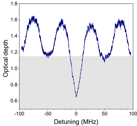
Fig. 3. Absorption profile of 200 MHz-section of a 6.4 GHz-wide AFC at \lambda=1532.05 nm and B=3 kG. The grey shaded area indicates remaining background absorption. The central dip is caused by unmodulated pump laser light.
