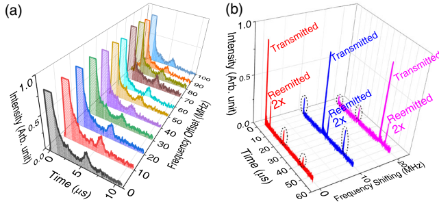
FIG. 4. Storage of data in multiple spectral modes. (a) Spectrally multiplexed AFC quantum memory used to simultaneously store optical pulses in 11 spectral modes for 5 \mu s. (b) Feed-forward mapping of spectral modes onto one with zero detuning. Laser pulses in three spectral modes were stored and reemitted after 5 \mu s. Frequency shifting using phase modulator PM3 allowed mapping any desired mode onto one with zero detuning. Only this mode was transmitted through the filter cavity. The reemitted pulses are magnified by a factor of 2, and crosstalk is indicated using dotted circles.
