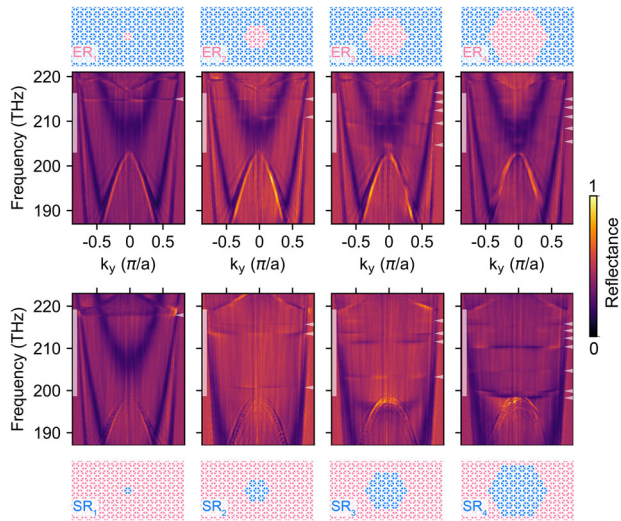
Figure 2. Dispersion versus cavity size. Experimentally retrieved dispersion diagrams of hexagonal cavities formed by patches of expanded-in-shrunk ( ER_n , upper row) or shrunken-in-expanded ( SR_n , lower row) unit cells, where n denotes the cavity's side length and the input is Y-polarized (no analyzer). Recognizable cavity modes as well as the bulk band gaps are highlighted by white pointers and light shaded bars, respectively, and the cavity geometries are depicted schematically.
