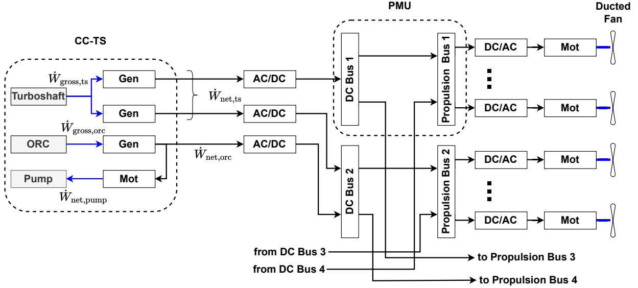
Figure 4: Dragon CC-TS powertrain architecture (adapted from Schmollgruber et al. [43]). Thick blue lines indicate mechanical power transmission, thick black lines electrical power transmission.
