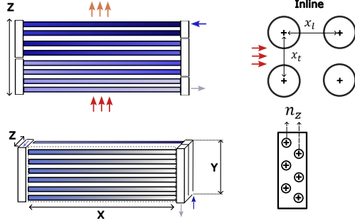
Figure 5: Evaporator core geometry: multi-pass inline bare tube bundle.
