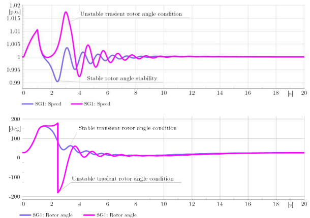
Fig. 6. Plot of rotor angle ( \theta ) and speed ( \omega ) of SG1 during a transient rotor angle stability. Stable condition when fault is cleared at t < t_{CFCT} = 0.977 sec and unstable at t > t_{CFCT} = 0.979 sec.
