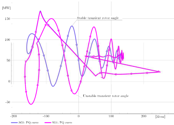
Fig. 8. Plot of active power versus reactive power (PQ plane) of SG1 during a transient rotor angle stability. Stable condition when fault is cleared at t = 0.977 sec and unstable at t = 0.979 sec.
