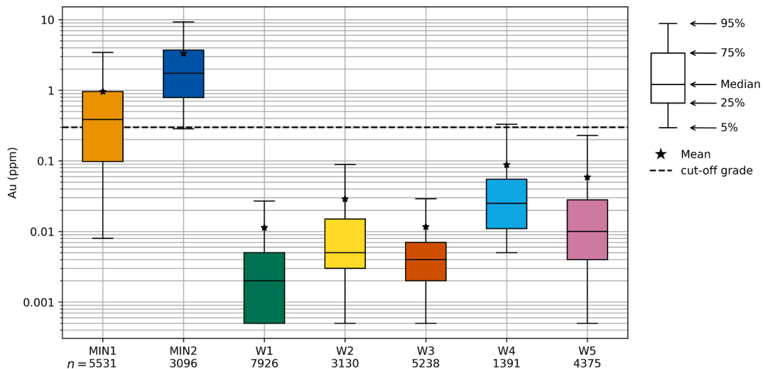
Fig. 8. Box and whisker plot of Au grade (ppm) for the clustering classes of Case Study I.
