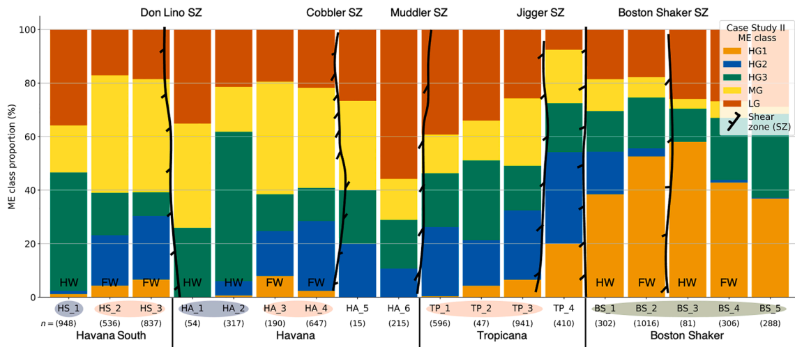
Fig. 15. ME class proportions (Case Study II) typically found in selected Tropicana Gold Mine orebody domains (x-axis). The shaded domains have roughly similar geochemical signatures. Also, see Fig. 14 for the spatial configuration, SZ = shear zone, HW = hanging wall, FW = footwall.
