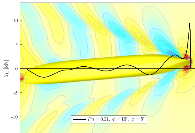
Figure 2.3.: Distribution of hydrodynamic sideforce, showing wave system (viewpoint is below the ship). Hull #34, leeway angle \beta = 5^\circ , heel angle \phi = 10^\circ . As the vessel heels, the fore and aft shoulders are brought close to the free surface, causing flow constriction and acceleration. This effect is especially pronounced at large heel angles ( \phi=10^\circ is normally adopted as operational limit for manned vessels).
