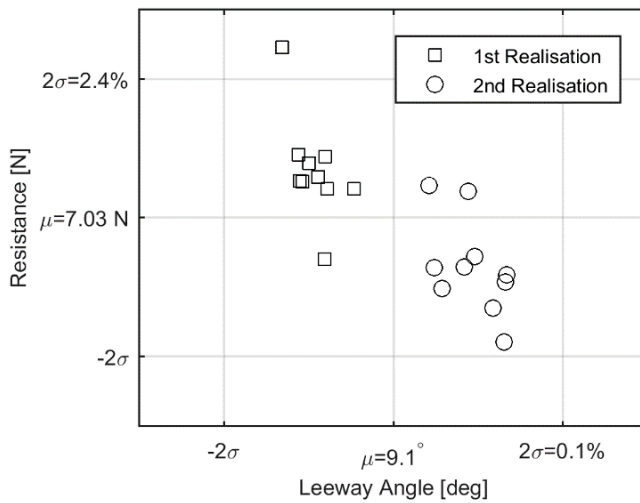
Figure B.14.: Complete set of repeat runs for precision limit for resistance n = 20 .
