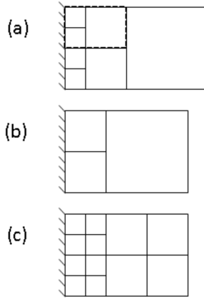
Figure B.1.: Illustration of the relationship between refinement level and refinement diffusion for mesh refinement.
