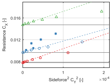
Figure A.9.: Data reduction for hull #4.
