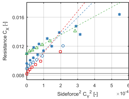
Figure A.14.: Data reduction for hull #45, parent of 3 rd Series.
