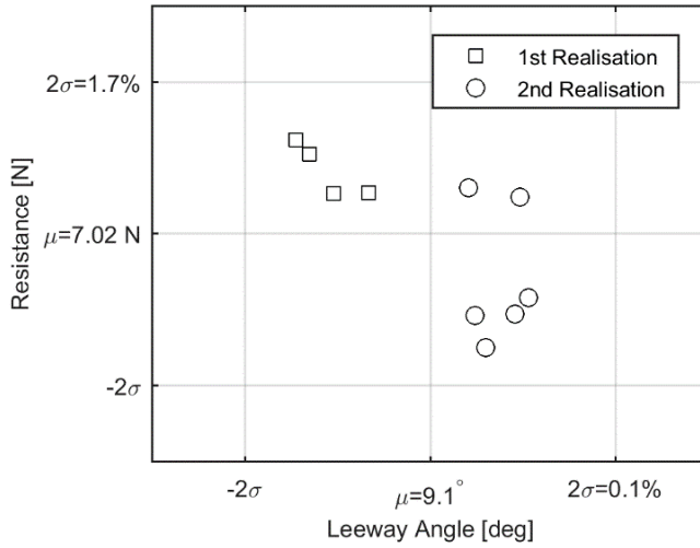
Figure B.13.: Precision limit of the alignment frame for resistance
