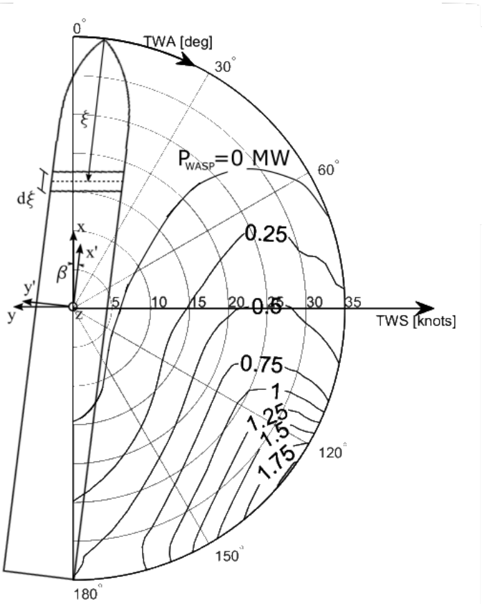
Figure 5.2.: Available wind-assist power, P_{WASP} . Installed main engine power = 1.3 MW Vessel coordinate system shown.
