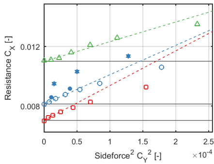
Figure A.12.: Data reduction for hull #7.
