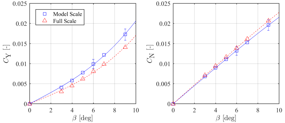
Figure 3.24.: Sideforce and yaw moment for full-scale and model-scale simulations of Hull #1, showing validation level for model-scale value. ( Fn = 0.168, \phi = 0^\circ ).
