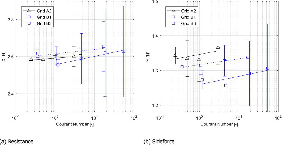
Figure 3.13.: Simulation U convergence for Courant number variation. ( \beta = 6^\circ ) U_T indicated with error bars.
