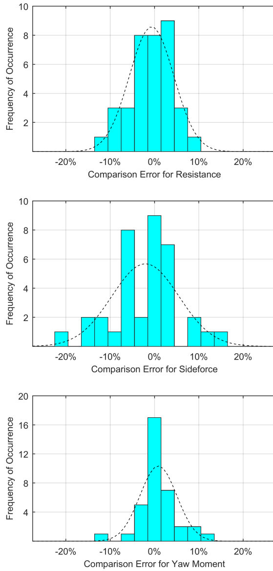
Figure 3.16.: E_{E_{ns}} for validation data set, using EASM turbulence model. \beta \neq 0^\circ ( n = 36 ).
