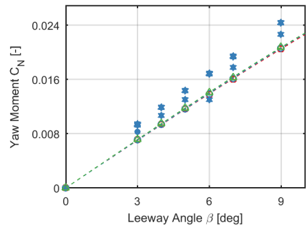
Figure A.6.: Data reduction for hull #1 (Parent hull of the 1 st Series).
