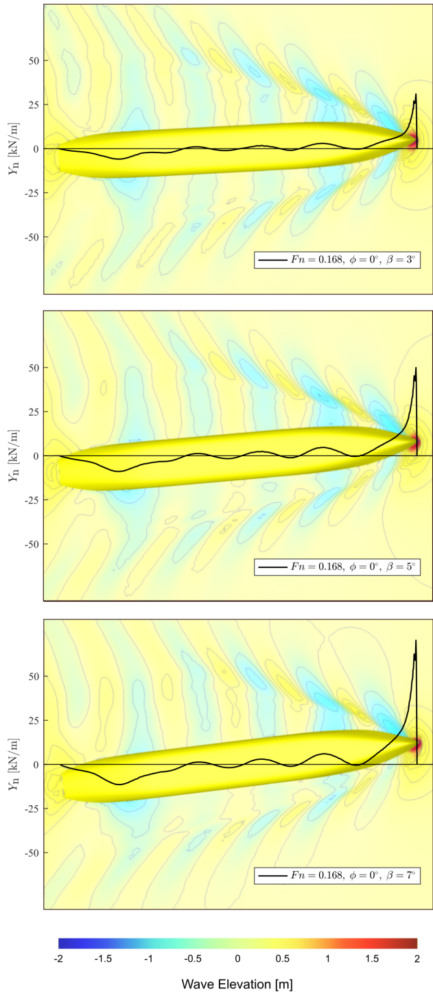
Figure 2.7: Distribution of hydrodynamic sideforce, showing wave system, for increasing leeway angle \beta . A low-aspect rectangular planform, such as a simplified hull form, develops a concentrated lifting force at the leading edge (Newman, 1977). The pressure peak increases with leeway angle \beta . This characteristic effect of low-aspect lift (Equation (2.4)) is the primary effect, and is apparently linear with leeway angle. The 'under-pressure' along the aft section is the so-called Munk moment, also a linear effect. Hull # 1, \phi = 0^\circ, F_n = 0.168 . Simulation result.
