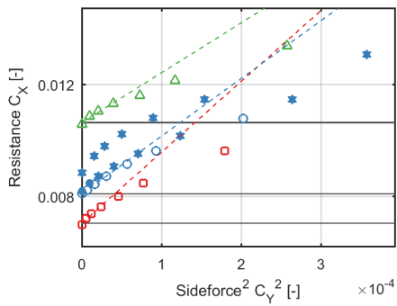
Figure A.13.: Data reduction for hull #34, parent of 2 nd Series.
