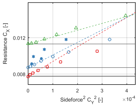
Figure A.11.: Data reduction for hull #6.
