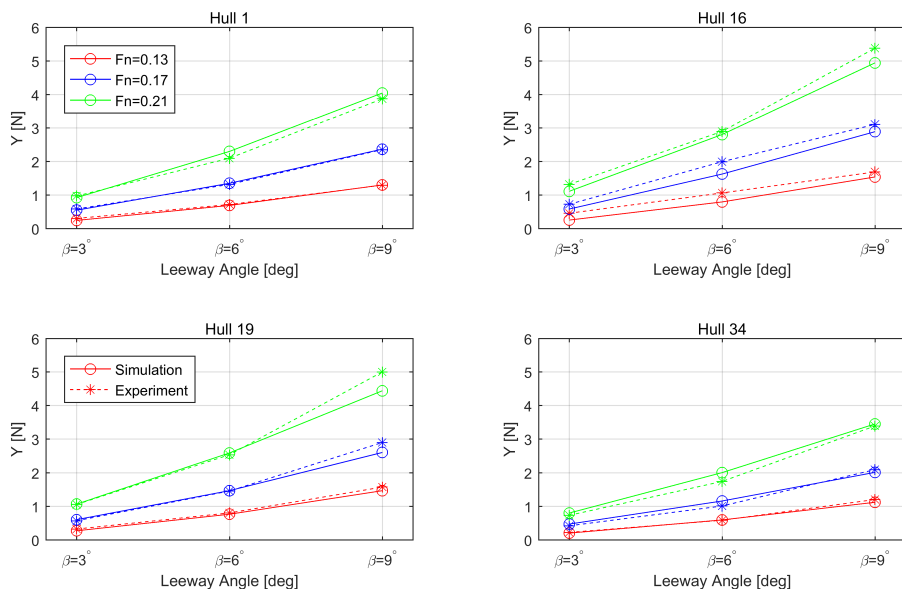
Figure 3.22.: Simulation and experimental results from the bare-hull validation set for sideforce.
