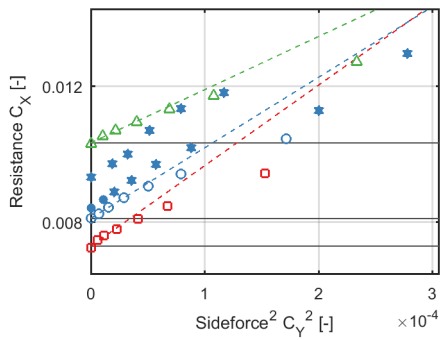
Figure A.10.: Data reduction for hull #5.
