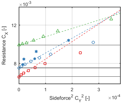
Figure A.7.: Data reduction for hull #2.
