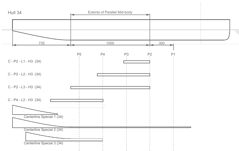
Figure 4.20.: Centreline-keel appendages
