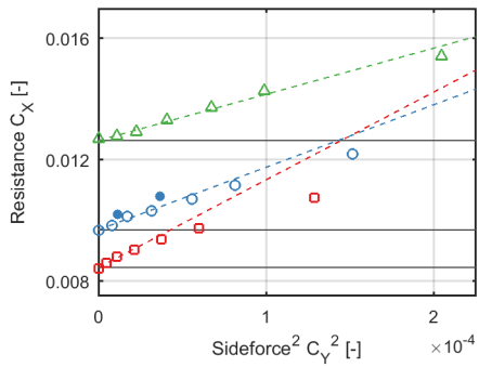
Figure A.8.: Data reduction for hull #3.
