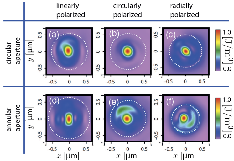
Fig. 14. Distorted energy densities obtained by focusing through the disk-shaped micro/nanoparticle with a misaligned real lens. The dashed white circle represents the projection of the disk-shaped particle on the detection plane.
