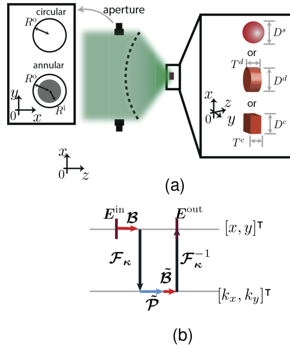
Fig. 1. (a) Schematic of focusing through a micro/nanoparticle by ideal lens. R^o is the radius of the aperture. R^i is the radius of the inner block. D^s denotes the diameter of the spherical particle. D^d denotes the diameter of the disk-shaped particle. T^d denotes the thickness of the disk-shaped particle. D^c denotes the lateral size of the cuboid particle. T^c denotes the thickness of the cuboid particle. (b) The corresponding field tracing diagram.
