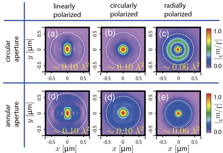
Fig. 7. Energy densities obtained by focusing the field through a disk-shaped micro/nanoparticle. The dashed white circle represents the projection of the disk-shaped particle on the detection plane.
