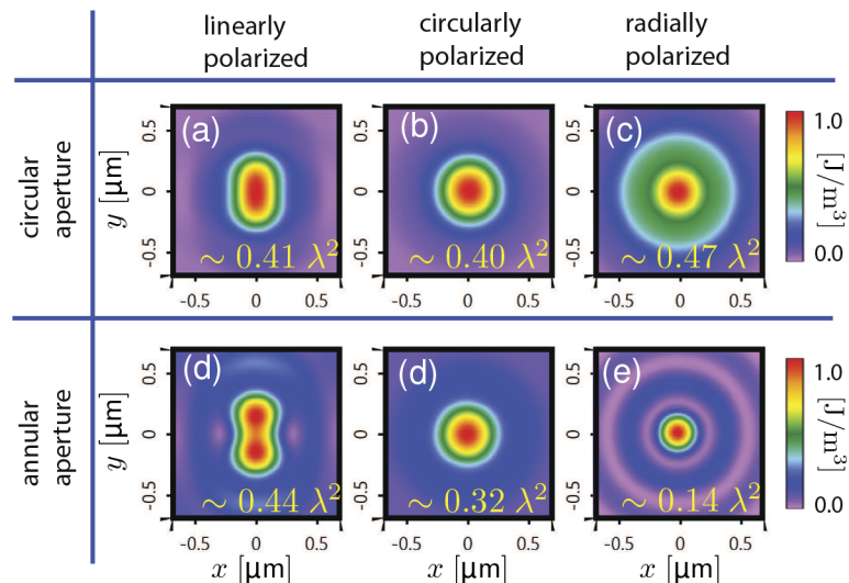
Fig. 8. Energy densities obtained by focusing the field through a planar slab which has the same thickness of the corresponding disk-shaped micro/nanoparticle in Fig. 7.
