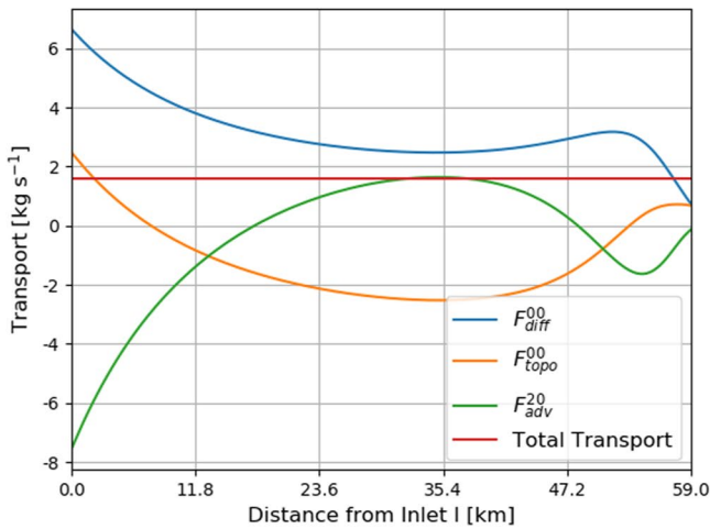
(c) E2–Transport Contributions
