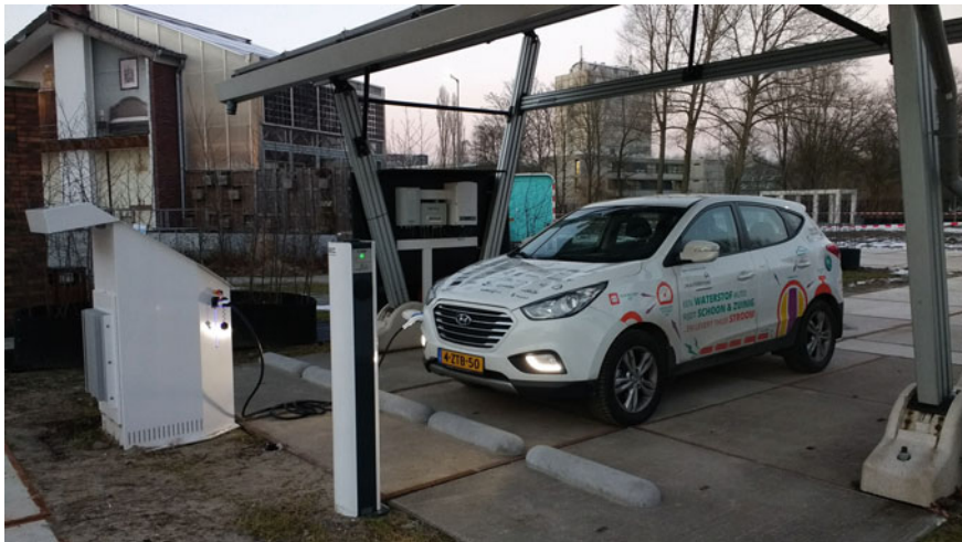
Fig. 8.3 Photo of the modified Hyundai ix35 FCEV connected to the grid through the V2G unit at The Green Village in The Netherlands
