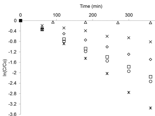
Figure 2.10. Effects of A/R ratio on degradation of phenol (2 mg/L, 0.1 M Na 2 SO 4 supporting electrolyte), photolysis ( \Delta ); A/R ratio (95/5) ( \diamond ); A/R ratio 85/15 ( \square ); A/R ratio 82/18 ( \times ); A/R ratio 74/26 ( \circ ); A/R ratio 50/50 ( \times )
