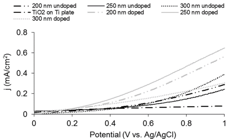
Figure 7.9. JV characteristics for the doped, undoped \text{BiVO}_4 and \text{TiO}_2 samples
