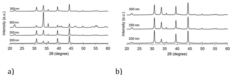
Figure 7.5. XRD pattern of samples of BiVO 4 a) undoped and b) 1 % W gradient doped on FTO. The dotted peaks represent the FTO peaks and the vertical lines represent the monoclinic scheelite peaks. The intensity of the XRD signal has been adapted to fit in the graph, but it must be noted that the signal of all the FTO peaks is approximately the same in all cases since the substrate is the same, and thus they must be taken as a reference.
