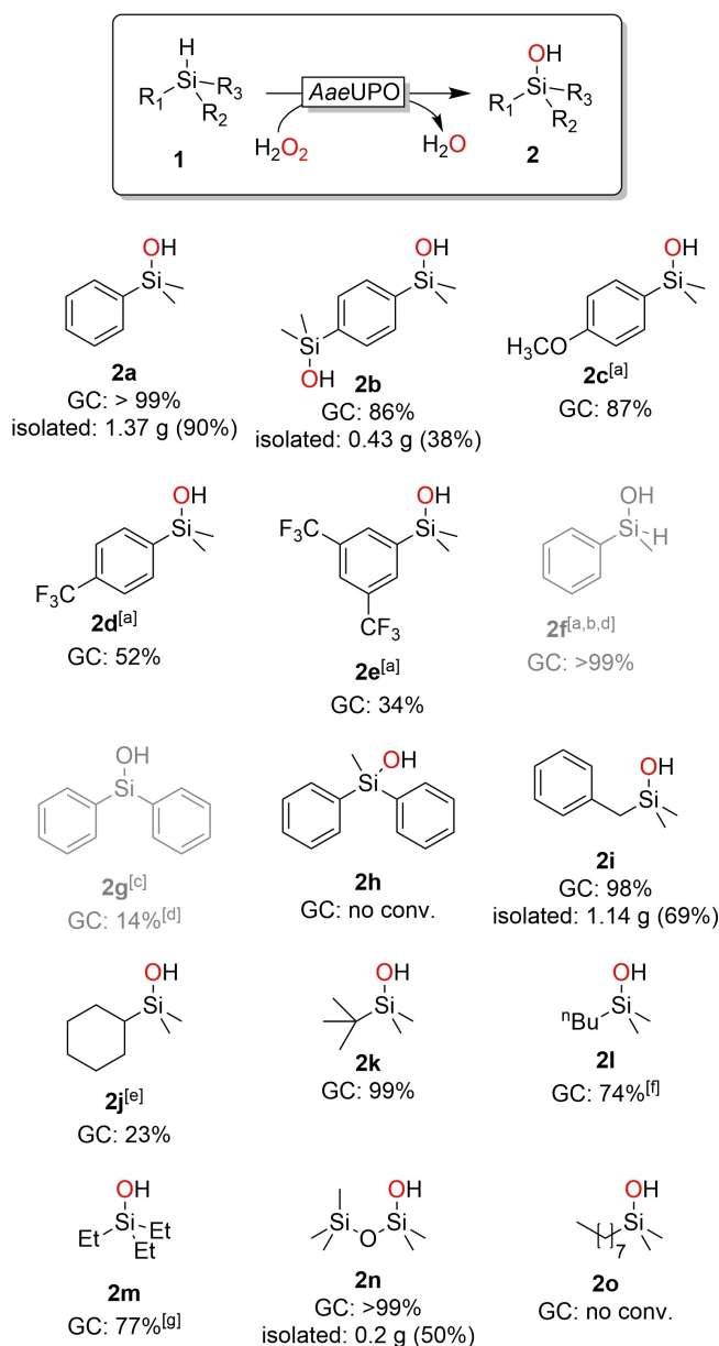
Figure 3. Substrate scope of AaeUPO -catalysed hydroxylation of organosilanes. General conditions: [Organosilane] = 50 mM, [ AaeUPO ] = 1 \mu\text{M} , buffer: 50 mM KPi pH 7.0 containing 30% (v/v) of acetonitrile, 25 ^\circ\text{C} , 600 rpm. The reaction was initiated by adding \text{H}_2\text{O}_2 (10 mM \text{h}^{-1} from a 1 M stock), 5 h. GC yields are given as averages of duplicate runs. For entries shown in grey, significant background conversion in the absence of AaeUPO was observed. [a]: significant amounts of dimerisation product observed; [b] negative controls showed approx. 45% conversion; [c] negative controls yielded the same conversion as in the presence of AaeUPO ; [d] both, mono- and dihydroxylation products were observed: silanediol:silanol = 6:1; [e] approx. equal formation of a yet non characterised C–H hydroxylation product; [f] approx. 26% of a yet non characterised C–H hydroxylation product; [g] approx. 12% of a yet non characterised C–H hydroxylation product.
