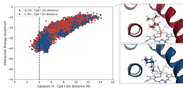
Figure 4. PELE simulation results for 1j ligand. (Left) The scatter plot shows the sampled poses' catalytic distance between the reactive oxygen in Cpd I and the silicon (blue) or carbon (red) reactive hydrogens (only the shortest distance between these two atoms is shown) against the enzyme-substrate interaction energy. The vertical dashed line marks a threshold of 4 Å for the catalytic distance. (Right) Snapshots of the catalytic poses show the positioning of the substrate with a carbon- (right top) or silicon- (right bottom) reactive catalytic distance (dashed lines).
