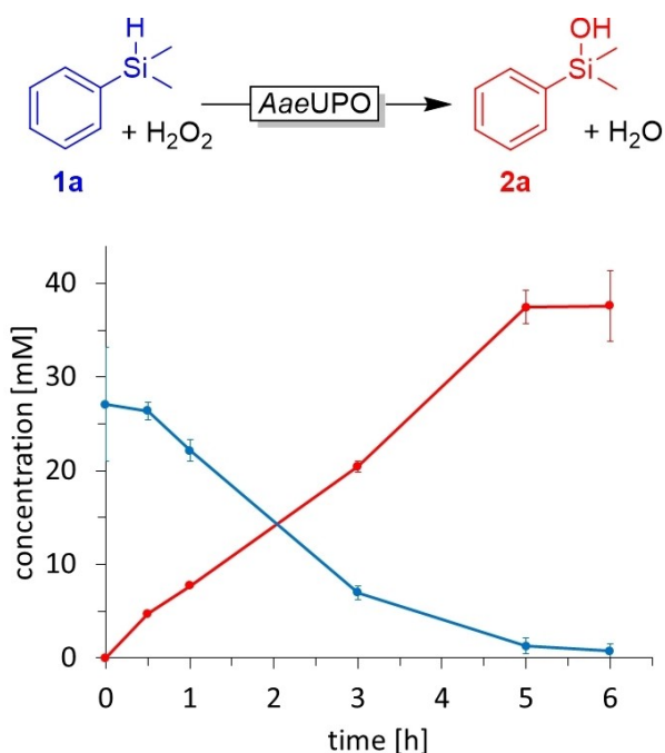
Figure 1. AaeUPO -catalysed hydroxylation of dimethylphenylsilane ( 1a ) to dimethylphenylsilanol ( 2a ). Conditions: [ 1a ] = 50 mM, [ AaeUPO ] = 1 \mu M, buffer: 50 mM KPi pH 7.0 containing 30% (v/v) of acetonitrile, 25 ^{\circ} C, 600 rpm, H 2 O 2 feeding-rate: 10 mM \times h -1 (from a 1 M stock). Please note that even in the presence of 30% (v/v) of acetonitrile, the starting material was not fully soluble explaining the lower than nominal initial concentration of 1a determined.
