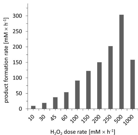
Figure 2. Influence of H 2 O 2 addition rate on the rate of the conversion of 1a to 1b . Conditions: [ 1a ] = 50 mM, [ AaeUPO ] = 1 \mu M, buffer: 50 mM KPi pH 7 containing 30% (v/v) of acetonitrile, 25 ^{\circ} C, 600 rpm. The reaction was initiated by addition of H 2 O 2 (10–1000 mM h -1 from a 1 M stock). Please note, the abscissa is not linear.
