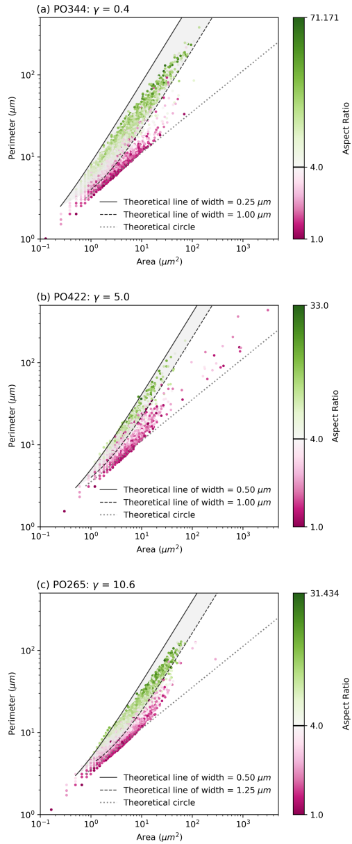
Figure A1. Filtering criteria for grain boundaries and pores.
