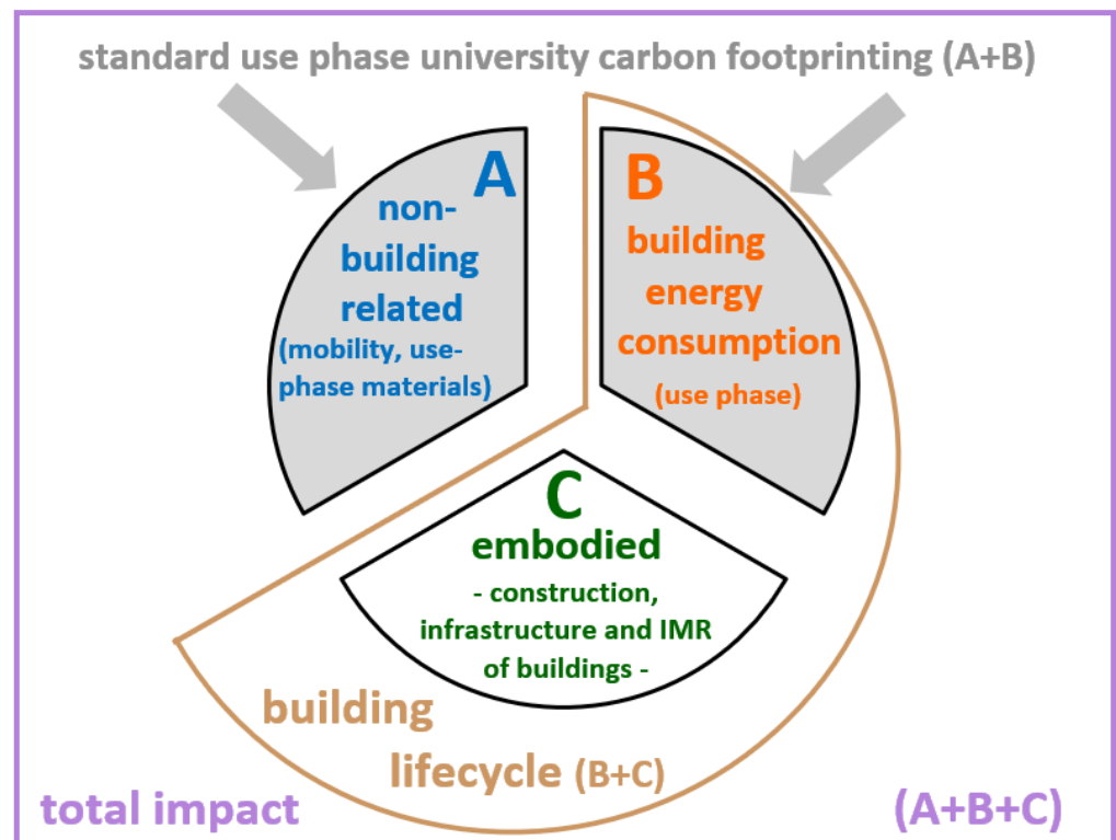
Figure 1. Composition of elements that make up the overall carbon footprint of a university. IMR = inspection, maintenance, repair.
