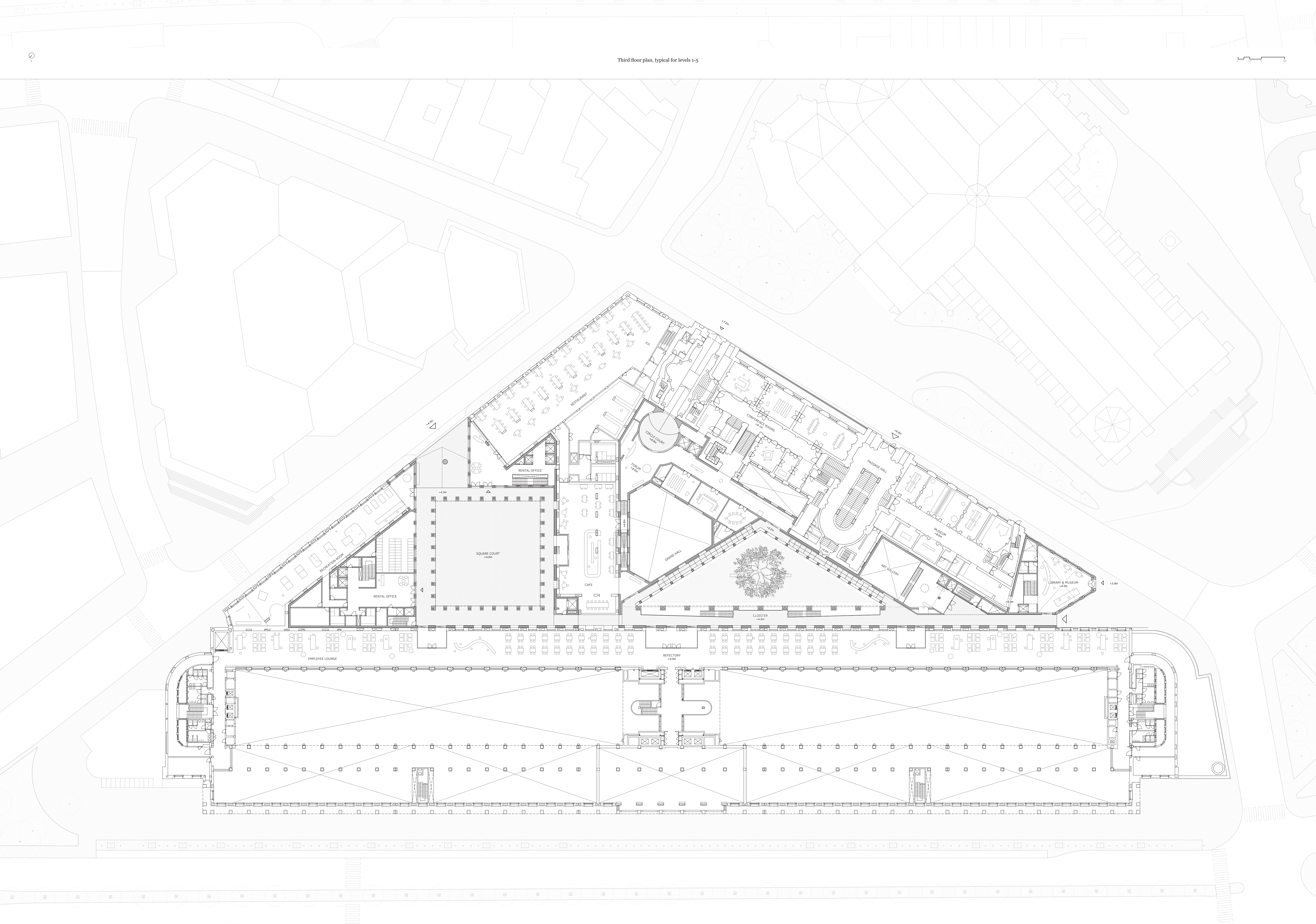
Upper ground floor, Bar & Book Storage
