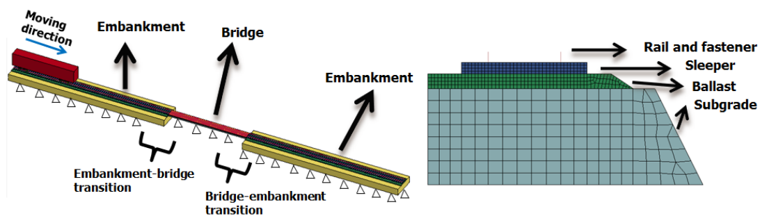
Figure 5: FE model of track transition zones.
