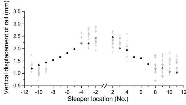
Figure 9: Comparison between measurements and simulation: black dots - simulation and cross - measurement results, from 57,58 .
