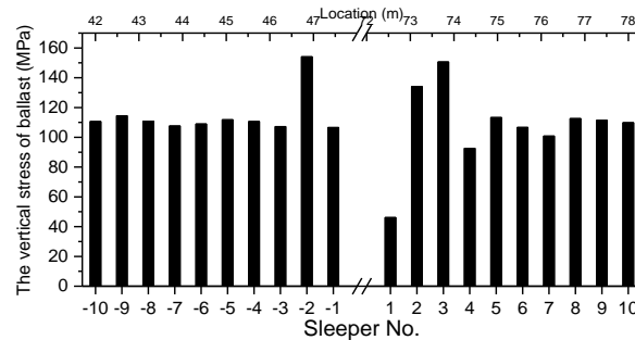
Figure 13: Ballast stress in the transition zone.
