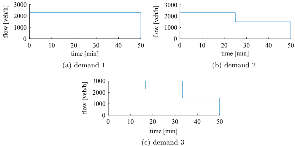
Fig. 6. Different demand profiles used in simulation.
