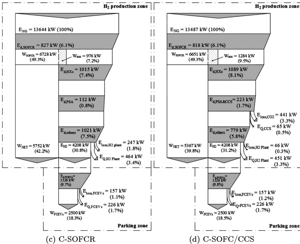
Fig. 6. Exergy flow diagrams of the four system designs in CaPP mode.
