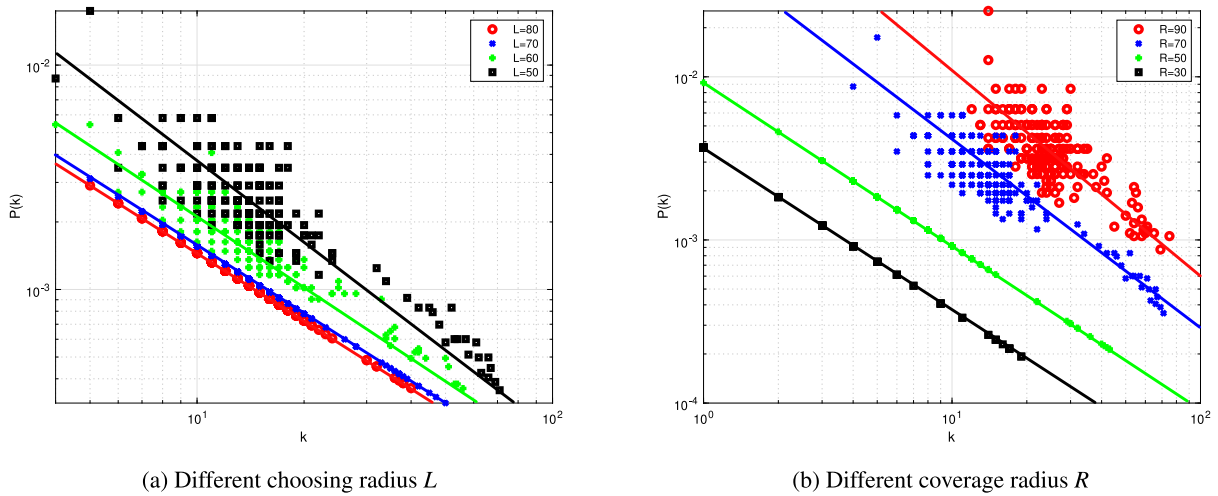
Fig. 5. Degree distribution comparison.
