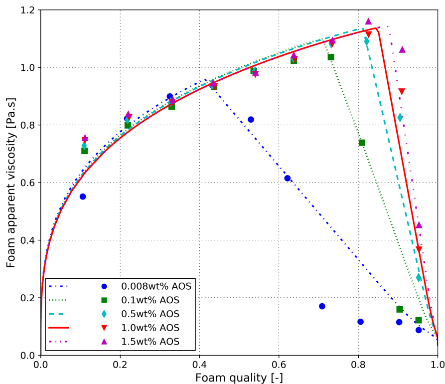
Figure 6 Simulation of the experimental data using F_2 and F_5 functions assuming constant set of parameters (Table 5) but different values of f_{mdry} (Table 6) to capture the effect of surfactant concentration.
