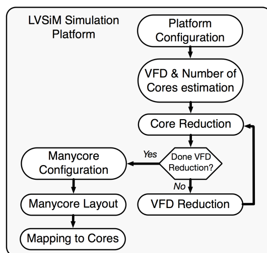
FIGURE 3. LVSIM simulation platform.
