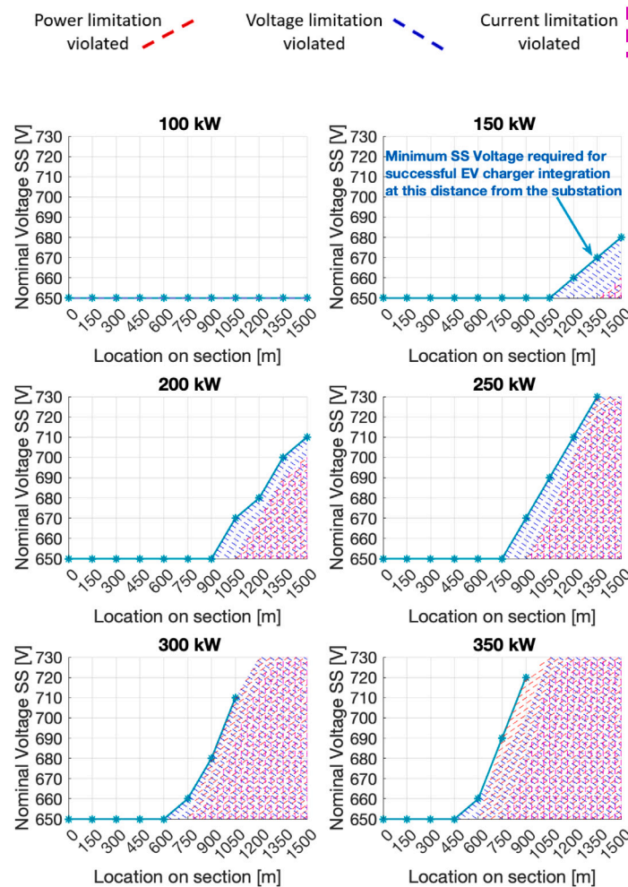
Fig. 6. The minimum substation voltage required for the successful EV charger integration of a certain size at any location on the section. The zone and type of the limiting grid violations are shown with dashed lines.
