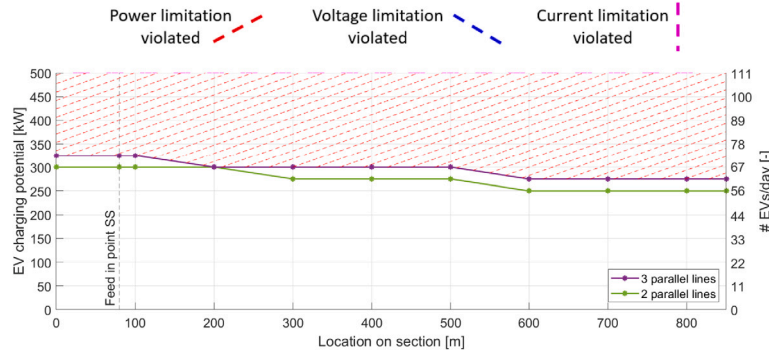
Fig. 10. Effect of adding extra paralleled overhead wire on the maximum achievable EV charging potential on section 23, day 268. The colored area indicates the limiting factor in the three paralleled overhead wire scenario.
