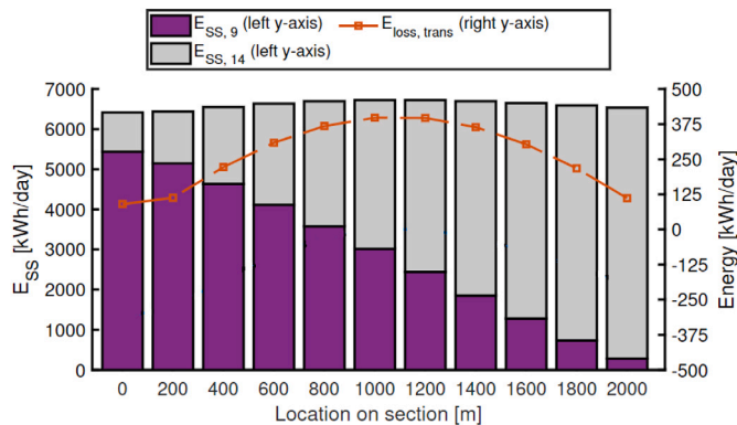
Fig. 14. Energy share of the two substations in supply zone A (left axis). A 400 kW EV charger is placed at different locations on sections 23 and 2. The orange line (right axis) shows the cables' energy losses due to transmission losses. (For interpretation of the references to color in this figure legend, the reader is referred to the web version of this article.)
