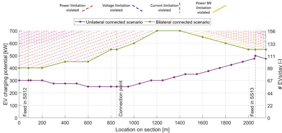
Fig. 12. Effect of introducing bilateral connections between sections 23 (left, 0–850 m) and 2 (right, 850–2150 m) on the maximum achievable EV charging potential.
