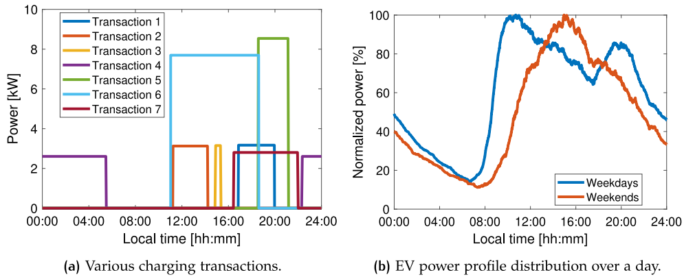
Fig. 4. The EV charging demand used in this paper from 1000 measured transactions in [47], (a) example of a few measured transactions, (b) summation curve of the 1000 transactions, normalized to a unity value.
