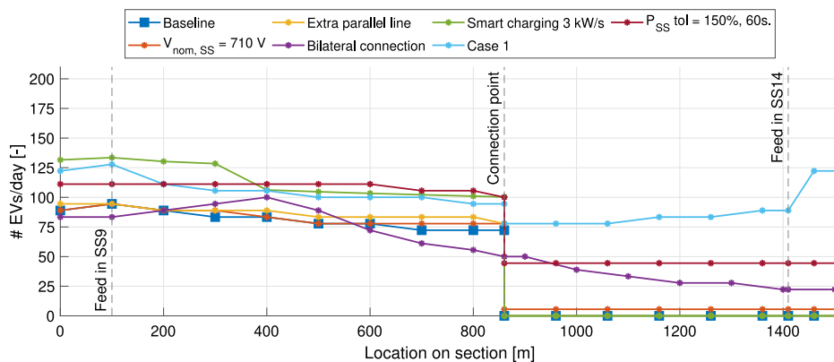
Fig. 16. Summary of the effect of various methods on the EV charging potential in supply zone B sections 25 and 26. Case 1: V_{nom, SS} = 710 V, an extra paralleled overhead line is added to the section, and the substation power rating is increased to 1100 kW.
