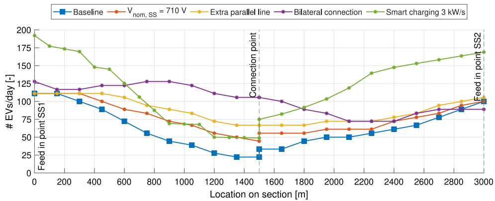
Fig. 9. Summary of various grid methods on the maximum achievable EV charging potential on the theoretical sections 111 (left) and 112 (right). Grid methods: increasing substation power and the multi-port converter are excluded from this graph as they showed no benefit.
