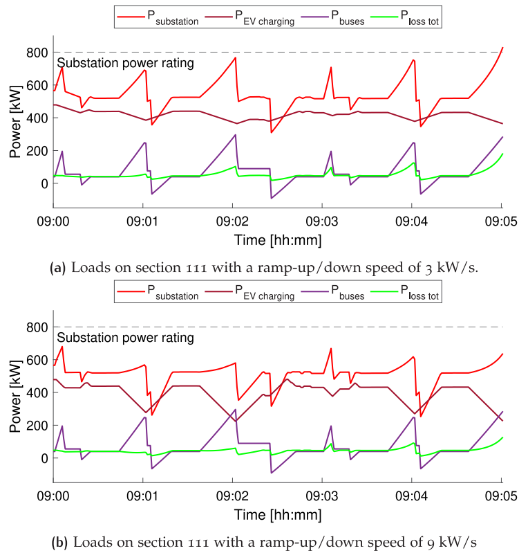
Fig. 8. The substation power (buses + EV + line losses) for an EV charger at 400 m. It is noticeable at 9:05 that the faster response of the management system allows the grid to avoid a power violation that occurs with the slower response.
