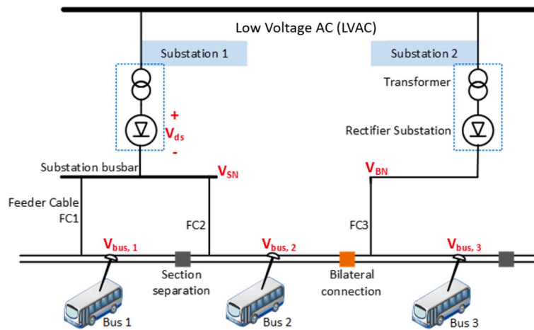
Fig. 2. The Trolleygrid and its components.
