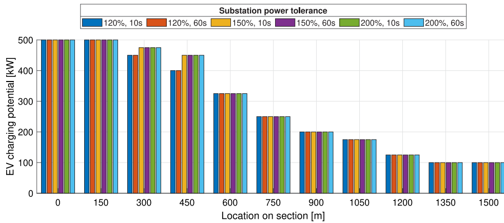
Fig. 7. Effect of various maximum substation power tolerances on the EV charging potential for section 111 for different charger locations: [Multiple of substation rated power, continuous violation duration].
