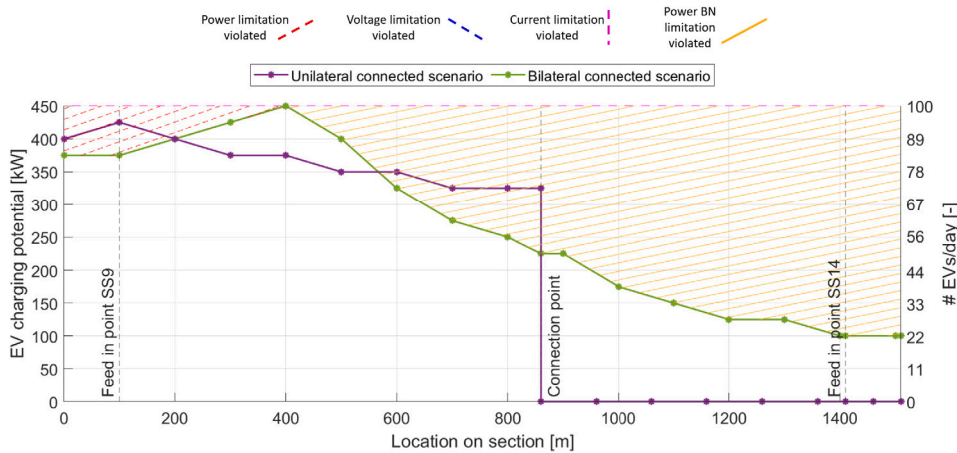
Fig. 13. Effect of introducing bilateral connections between sections 25 (left, 0–860 m) and 26 (right, 860–1510 m). The power limitation at the bilaterally connected substation P_{BN} is also shown.
