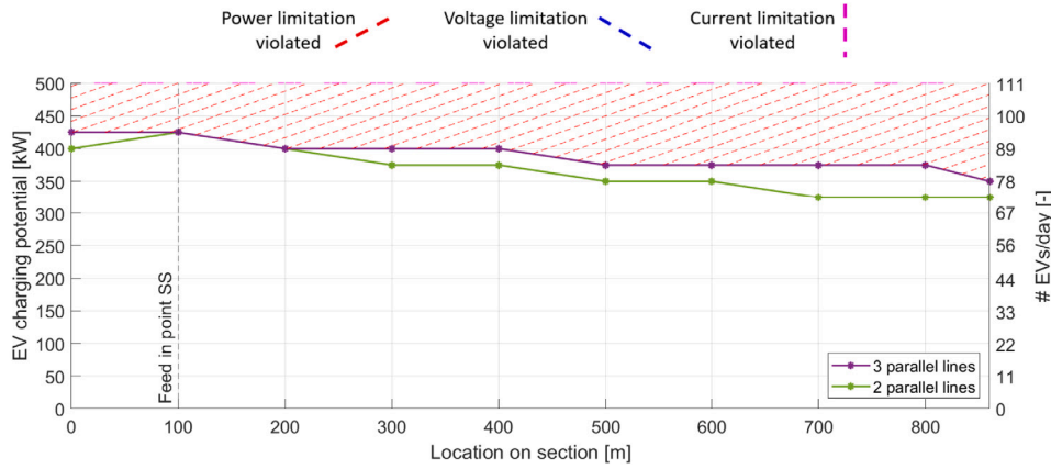
Fig. 11. Effect of adding extra paralleled overhead wire on the maximum achievable EV charging potential on section 25, day 268. The colored area indicates the limiting factor in the three paralleled overhead wire scenarios.
