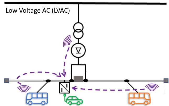
Fig. 3. Illustration of Fleet-Aware Smart Charging: In this method, the substation and the vehicles on the section communicate their states to the EV charger (power, voltage, location) and the latter computes its allowable charging power that would not break any of the grid limitations at any node on the line (not just at the charger).
