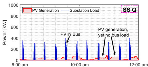
Fig. 1. Simulation results showing the mismatch between solar PV generation and substation demand in the trolleygrid of Arnhem [8].
