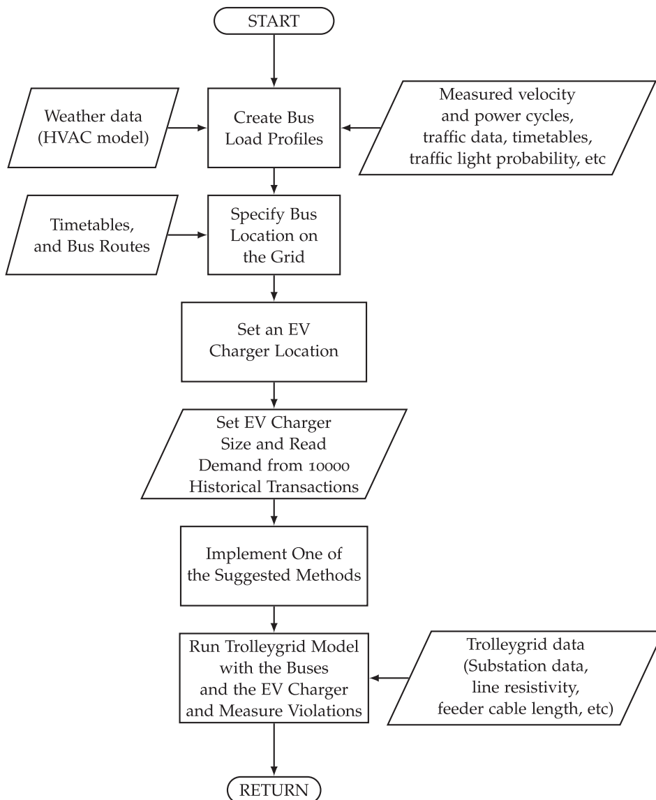
Fig. 5. Flowchart of the trolleygrid model with the EV charger.
