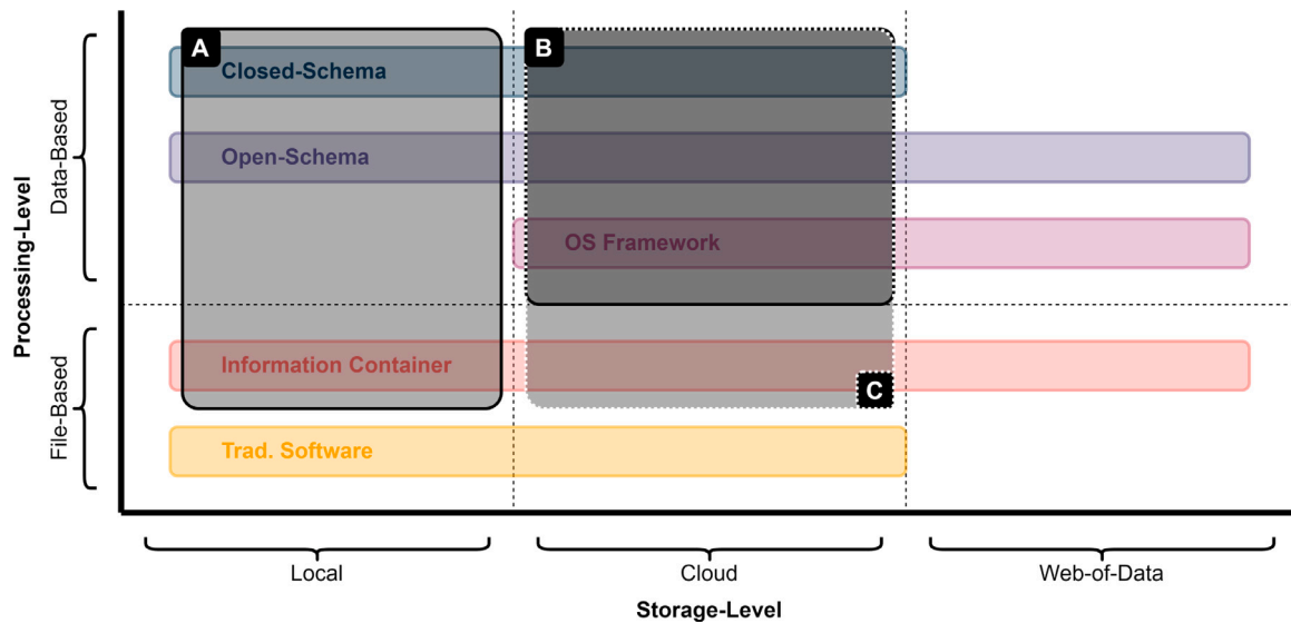
Fig. 4. The framework can help categorize data management concepts as a combination of the identified categories to improve the understanding of data management approaches in construction informatics, e.g for different implementations of the BIM concept (A/B), or similar implementation of two concepts, such as BIM (B) and CDE (C).
