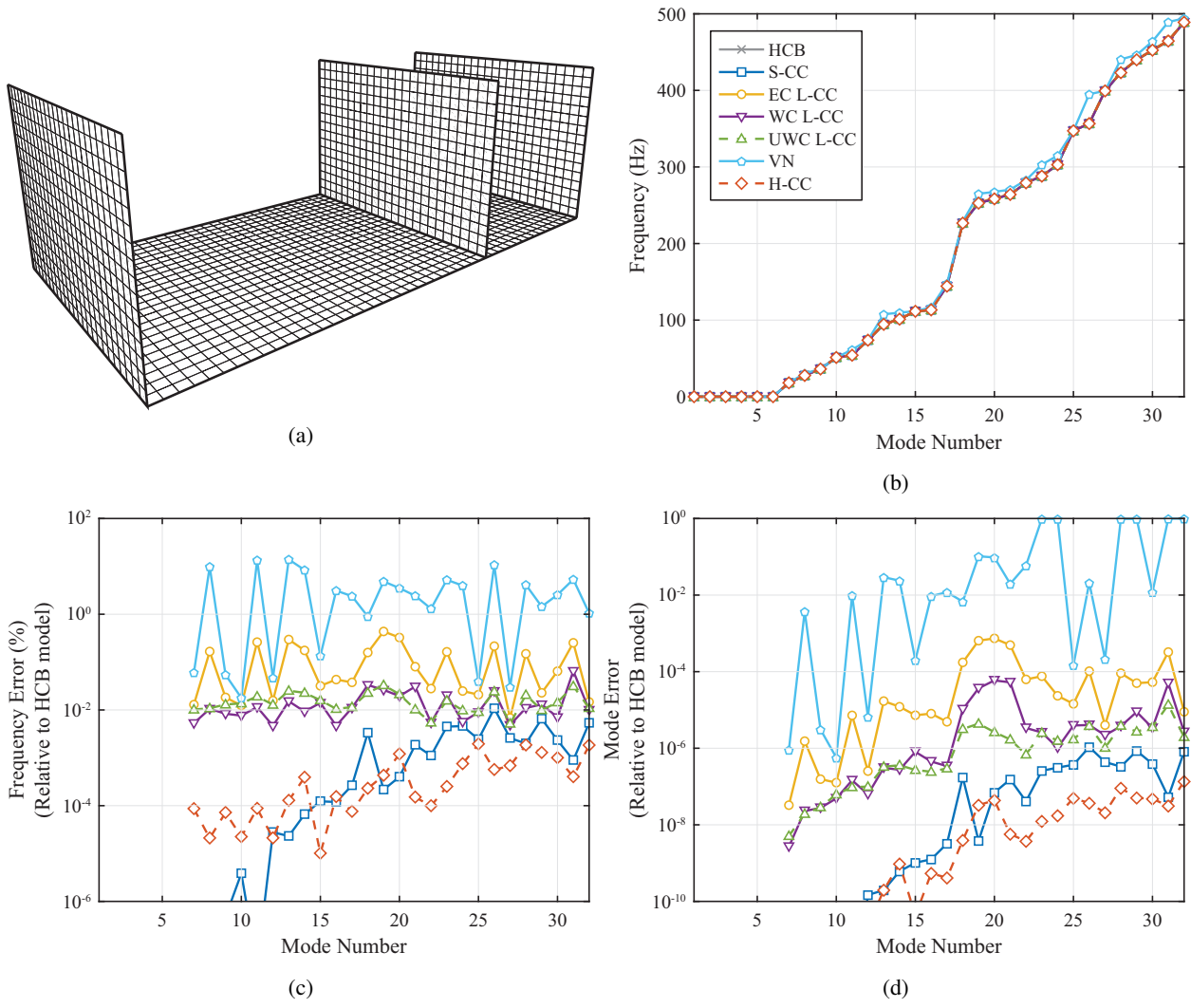
Figure 5: FE mesh (a), natural-frequency comparison (b), frequency-error comparison (c), and mode-error comparison (d) for the W-bracket model.
