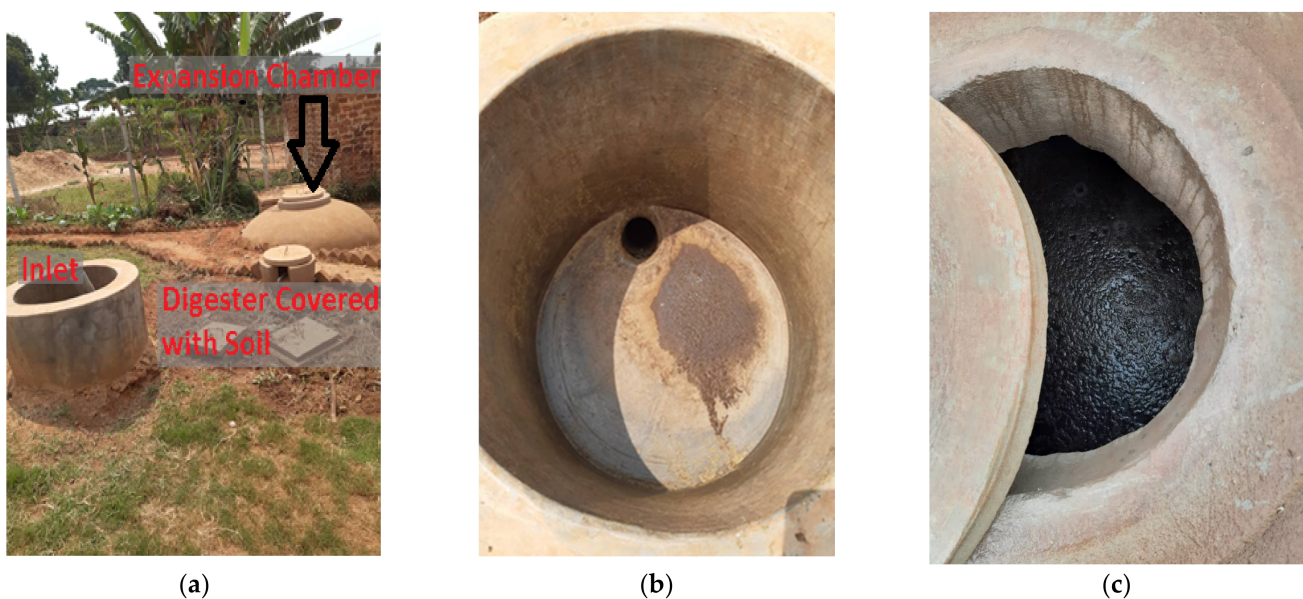
Figure 6. (a) Side view of the expansion chamber and inlet (b) Aerial view of the inlet and (c) Aerial view of open expansion chamber with slurry exposed to ambient conditions.
