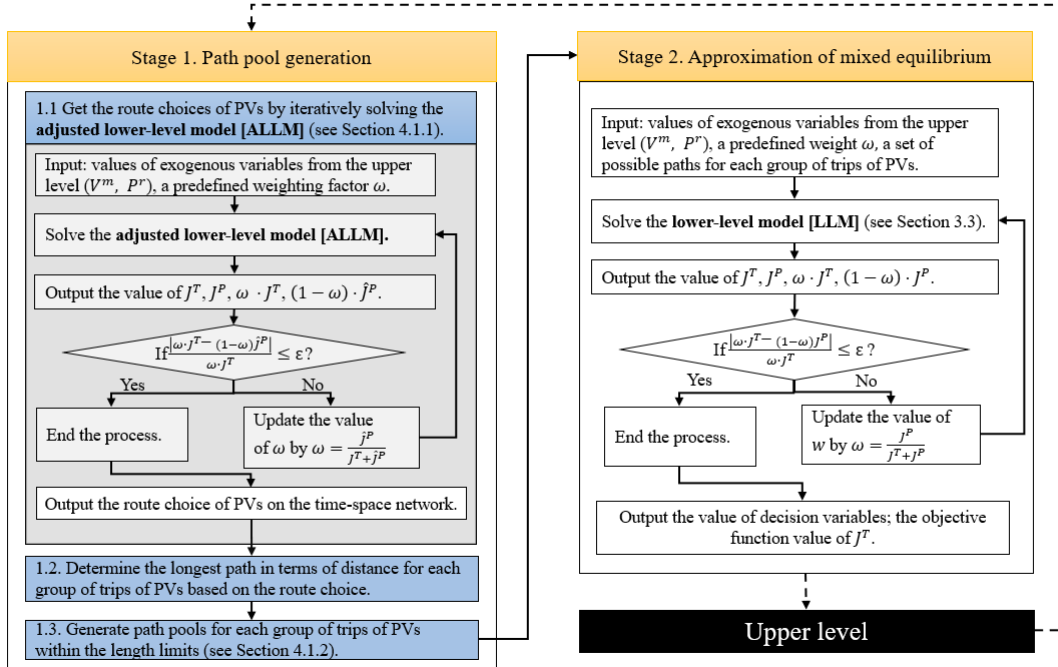
Figure 3.2: Framework of the lower-level solution method.
