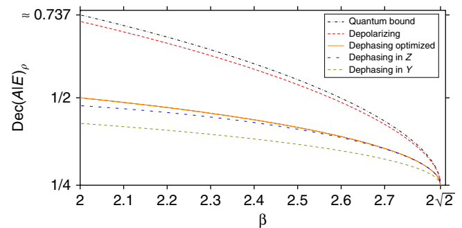
Figure 5 | Comparison of the quantum bound with the actual values of \text{Dec}(A|E)_\rho for some example channels and measurements. The black dash-dotted line on top shows the quantum bound, that is, the maximal value of \text{Dec}(A|E)_\rho that is compatible with a measured CHSH value \beta in quantum theory. The other four plots are parametric plots: The parameter that is varied is the noise parameter of the channel (see Supplementary Notes 2 and 5). For each noise parameter, the value of \text{Dec}(A|E)_\rho of the resulting state is calculated, as well as the CHSH value \beta that one would measure for this state using the standard measurements in the X - Z -plane that would be optimal for an EPR pair. This measurement happens to be optimal for the resulting state for the depolarizing channel, but not for the dephasing channels. The orange solid line also shows such a parametric plot for the dephasing channel, but for that line, the CHSH value \beta is not calculated for the standard measurement for the EPR pair but for the measurement that is optimal for the actual resulting state 50 . The resulting curve is independent of the dephasing direction.
