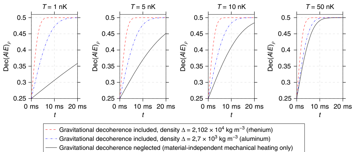
Figure 8 | Predicted values of the decoherence quantity in the optomechanical experiment. This figure shows the predicted values of \text{Dec}(A|E)_{\rho} as a function of the running time of the optomechanical experiment for different temperatures and for different materials of the mechanical element as calculated in the proposed model for gravitational decoherence. In addition, \text{Dec}(A|E)_{\rho} is plotted for the case where gravitational decoherence is not taken into account. When the gap between the predicted values with and without gravitational decoherence is large enough, the decoherence estimation formalism allows for a test that potentially falsifies the proposed model for gravitational decoherence. The calculations have been made for the example experimental parameters g_0 = 1 \text{ s}^{-1} , \omega_m = 1 \text{ s}^{-1} and \gamma_m = 10^{-10} \text{ s}^{-1} .
