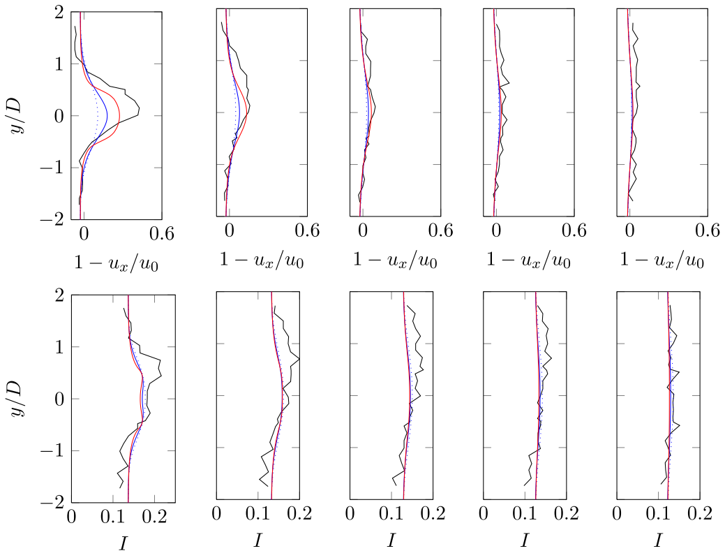
Fig. 21. Lateral velocity deficit and turbulence intensity profiles for the Fluidity simulations vs Mycek et al. at x = 2D, 4D, 6D, 8D and 10D for the upstream turbine with I_\infty = 15\% , C_T = 0.75 and u_{in} = 0.83 \text{ ms}^{-1} . The same legend as in Fig. 10 is used.
