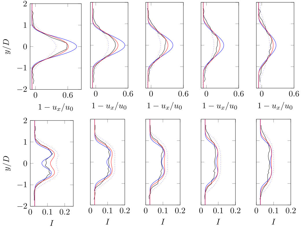
Fig. 22. Lateral velocity deficit and turbulence intensity profiles for the Fluidity simulations vs Mycek et al. at x = 2D, 4D, 6D, 8D and 10D for the downstream turbine with I_\infty = 3\% , C_T = 0.81 and u_{in} = 0.80 \text{ ms}^{-1} . The same legend as in Fig. 10 is used.
