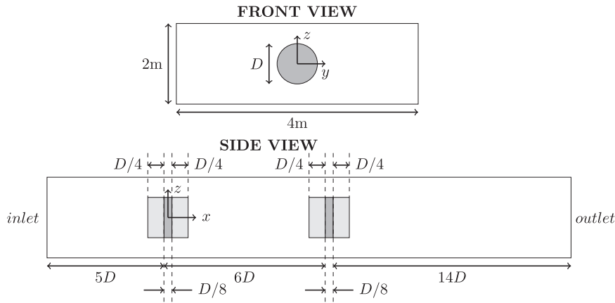
Fig. 17. Numerical domain with D=0.792 m used in the Fluidity simulations of the Mycek et al. experimental setup with x , y and z pointing in the streamwise, lateral and vertical directions respectively. The dark grey area represents the actuator discs and the light grey area around the discs represents the locations where the additional \omega source term, Eq. (9), is applied.
