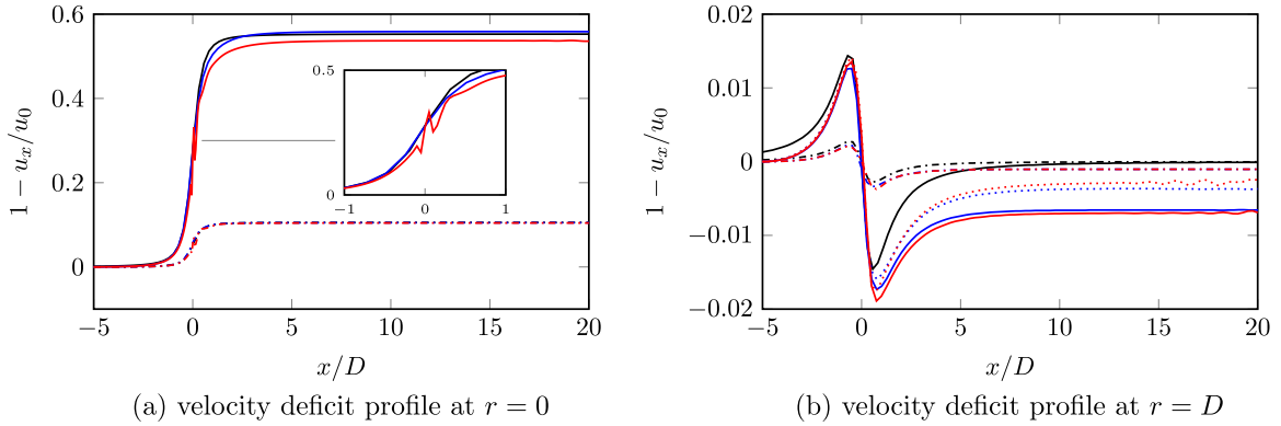
Fig. 3. Streamwise comparison velocity deficit plots with Re = 6.0 \times 10^7 . The Conway solution is shown in black ( C_T=0.2 (---) and C_T=0.8 (—)). The Fluidity results are shown in blue ( C_T=0.2 (---) and C_T=0.8 (—)) and the OpenFOAM results are shown in red ( C_T=0.2 (---) and C_T=0.8 (—)). The dotted lines in (b) correspond to simulation results using a larger computational domain of 25D \times 20D \times 20D instead of the usual 25D \times 10D \times 10D domain described in Fig. 2.
