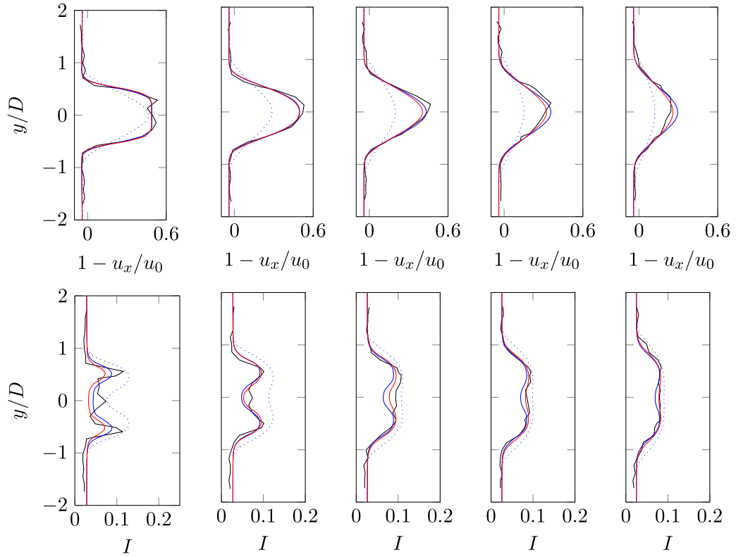
Fig. 20. Lateral velocity deficit and turbulence intensity profiles for the Fluidity simulations vs Mycek et al. at x = 2D, 4D, 6D, 8D and 10D for the upstream turbine with I_\infty = 3\% , C_T = 0.81 and u_{in} = 0.80 \text{ ms}^{-1} . The same legend as in Fig. 10 is used.
