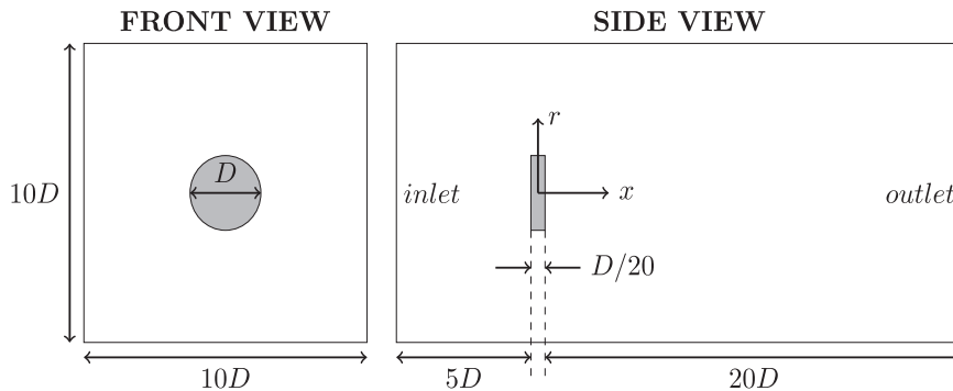
Fig. 2. Numerical domain with D = 20 \text{ m} used in both Fluidity and OpenFOAM simulations corresponding to the comparison plots presented in Figs. 3 and 4. The dark grey area represents the actuator disc.
