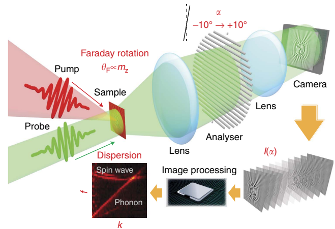
Figure 1 | Schematic illustration of spin wave tomography. Spin-wave tomography (SWaT) is based on the observation of the propagation dynamics of spin waves with the pump-and-probe magneto-optical imaging method. Various modes of spin waves are excited simultaneously by the illumination of the pump laser pulse in magnetic materials. The propagation dynamics of the spin waves are measured through the Faraday effect on the probe pulse ( \theta_F ), which is proportional to the magnetization along the direction normal to the sample surface ( m_z ). The images of \theta_F are obtained by analyzing the transmission images ( I(x) ) observed at various angles of the analyzer ( \alpha ) 26 . The spin-wave dispersion relations are reconstructed by Fourier transforming the propagating waveform of the spin waves.
