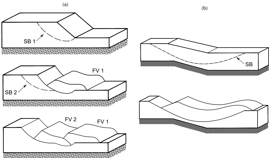
Figure 5.1: a) scheme of a retrogressive failure, and b) scheme of a translation failure (after Locat et al. 2011)
