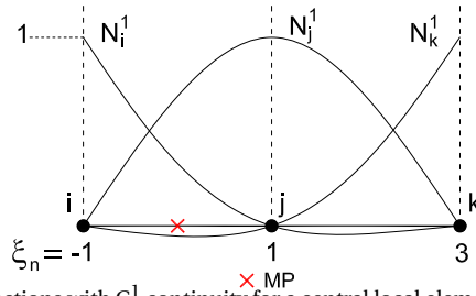
Figure 3.17: CPM shape functions with C^1 continuity for a central local element
