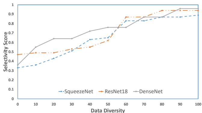
Fig. 2. Selectivity Score on Biased-Car dataset wrt data diversity
