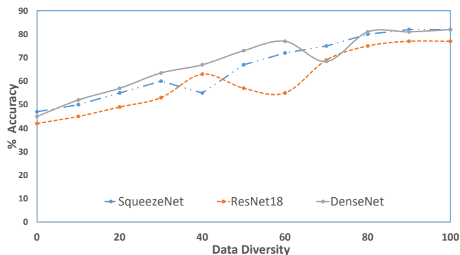
Fig. 3. Accuracy on Biased-Car dataset wrt data diversity
