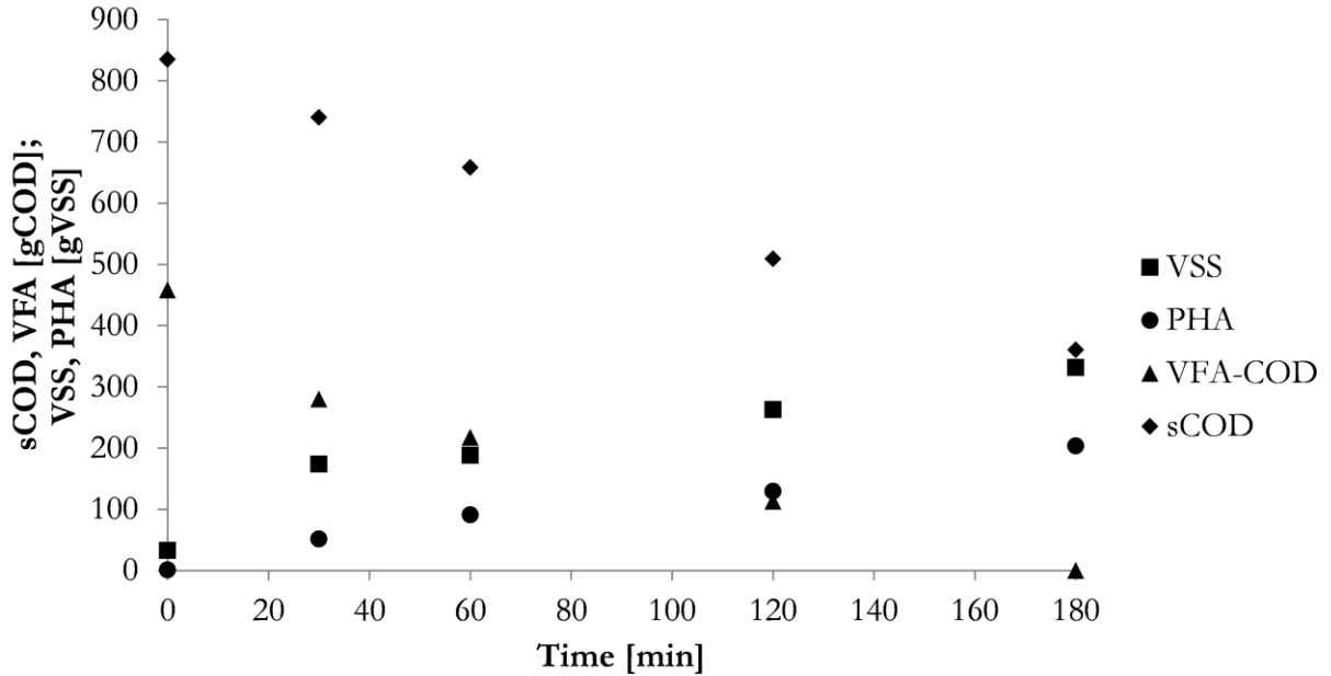
Figure 5. Detailed characterization of a PHA accumulation potential experiment (15-08-2017). Illustrating the evolution of \text{COD}_{\text{Sol}} , \text{COD}_{\text{VFA}} , PHA and VSS over time in absolute amounts.
