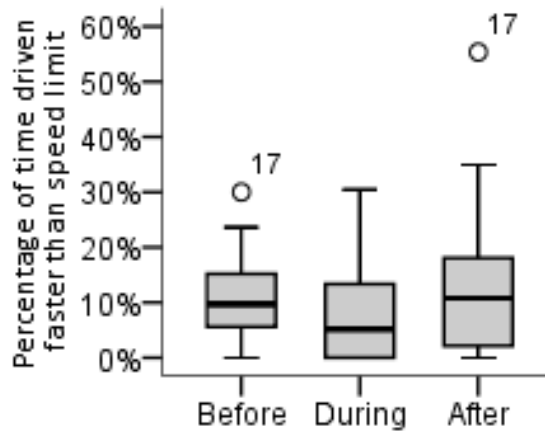
Figure A3: Percentage of time participants drove above the speed limit, 6 seconds before, during, and 6 seconds after they visually-manually operated the navigation system. The dots marked '17' represent outliers (by one participant); the boxplots show minimum, first quartile, median, third quartile and maximum.
